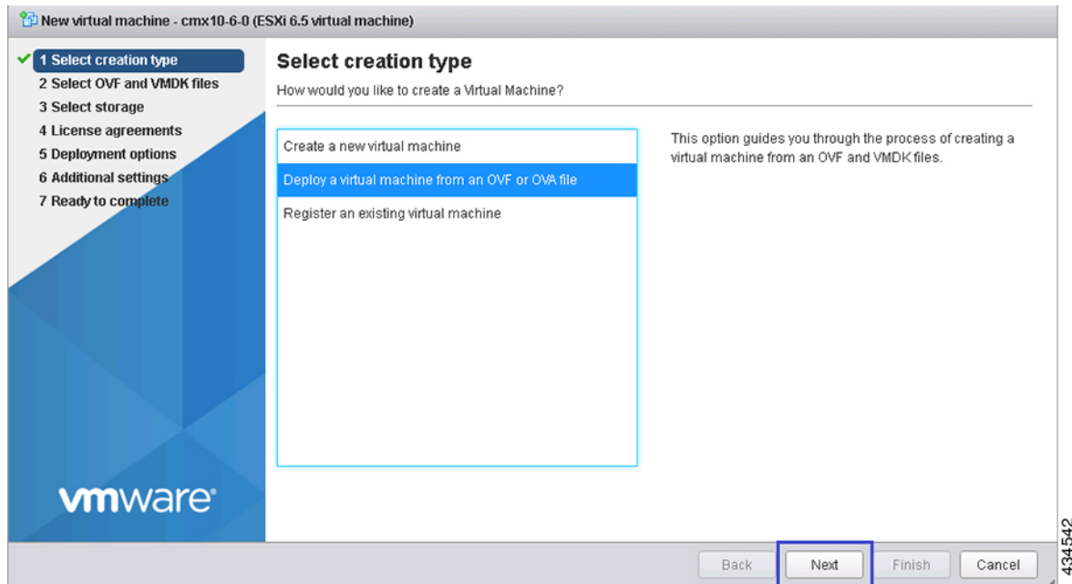
Figure 2: Deploy VM
