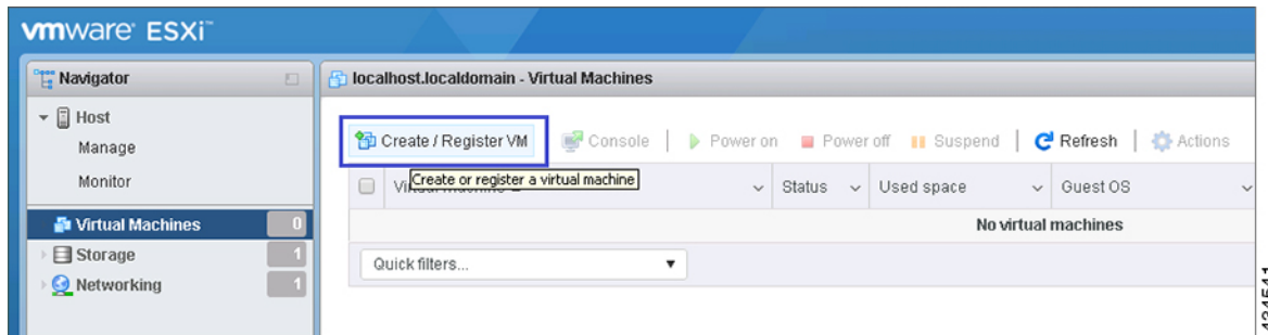
Figure 1: Create/Register VM
