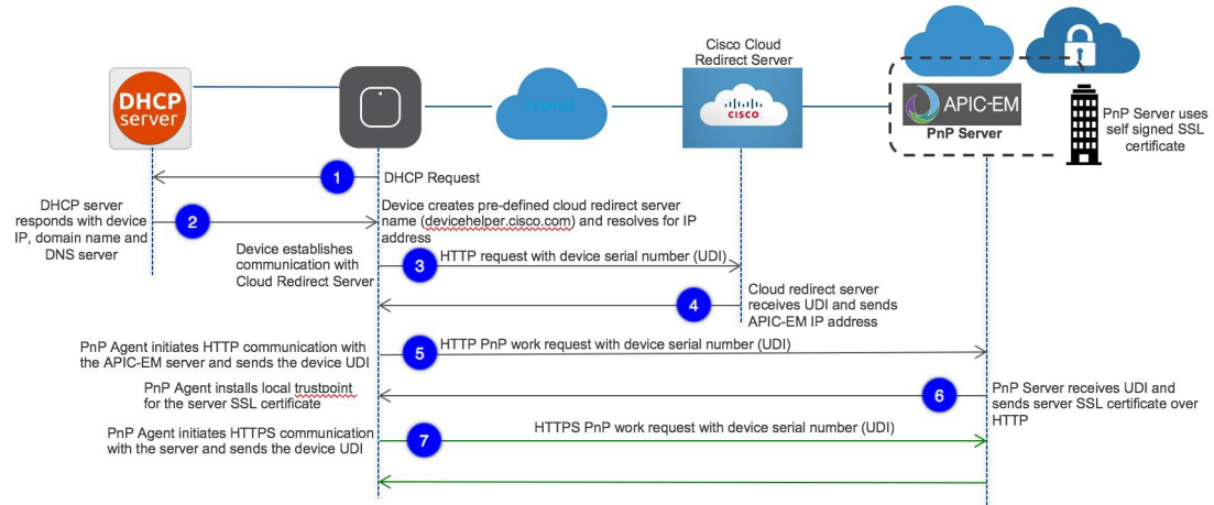
Figure 2: Cloud Plug and Play Device Redirect to APIC-EM controller flow
