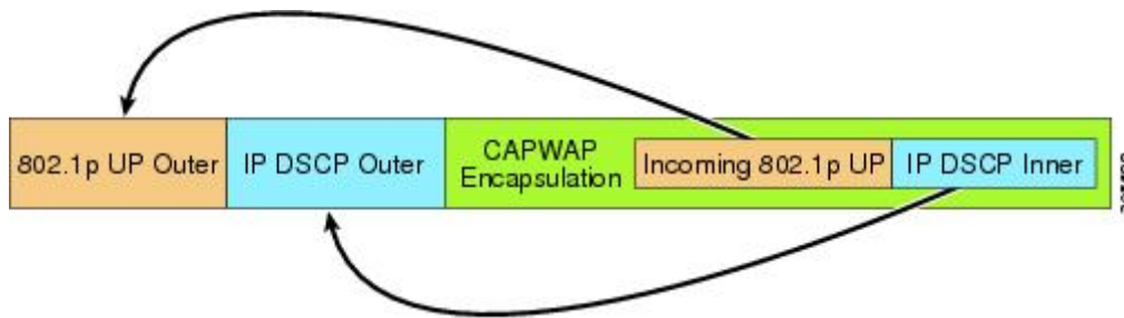
Figure 22: Controller to RAP Path
