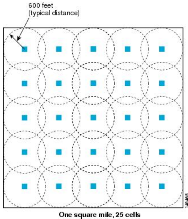
Figure 7: Cell Radius of 600 Feet and Access Point Placement for Nonvoice Mesh Networks
