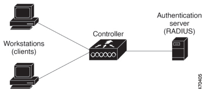
Figure 3: Local Web Authentication Device Roles
