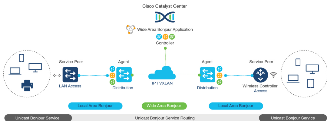
Figure 27: Overlay Bonjour Service for a BGP EVPN-Enabled Enterprise Network
