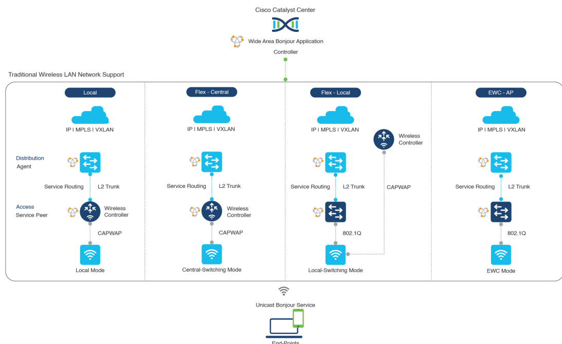
Figure 24: Enterprise Traditional Wireless LAN Network Design
