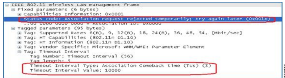
Figure 20: Association Reject with Comeback Time
