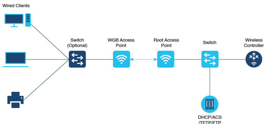
Figure 14: Example of a WGB
