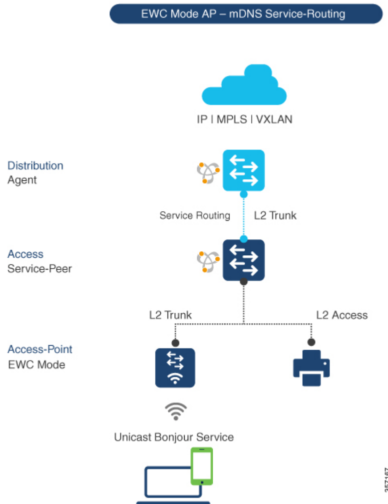
Figure 30: Cisco Catalyst Switch and EWC Mode Access Point
