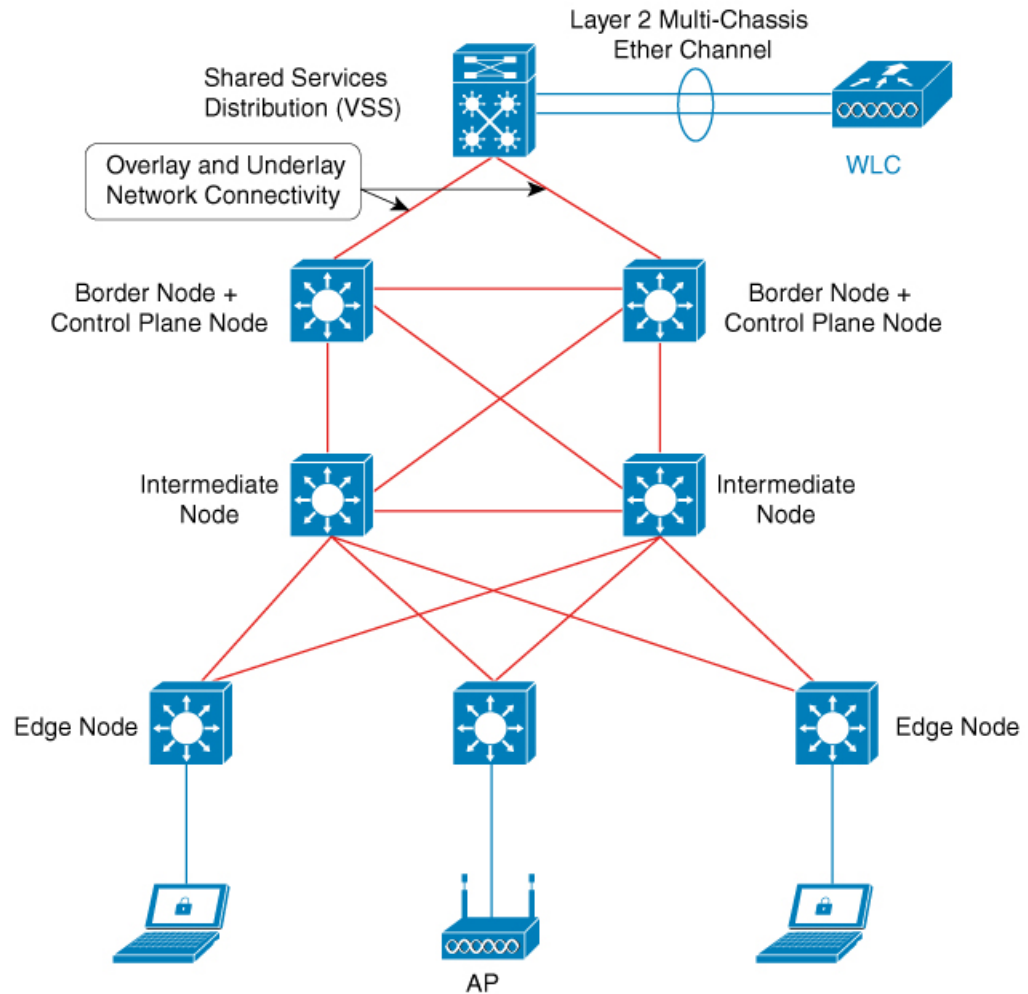
Figure 13: SD-Access Wireless
