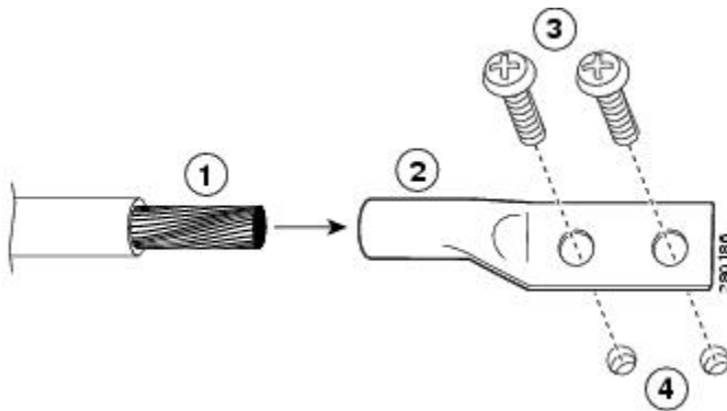
Figure 4: Attaching a Grounding Lug to the Chassis Ground Connector
