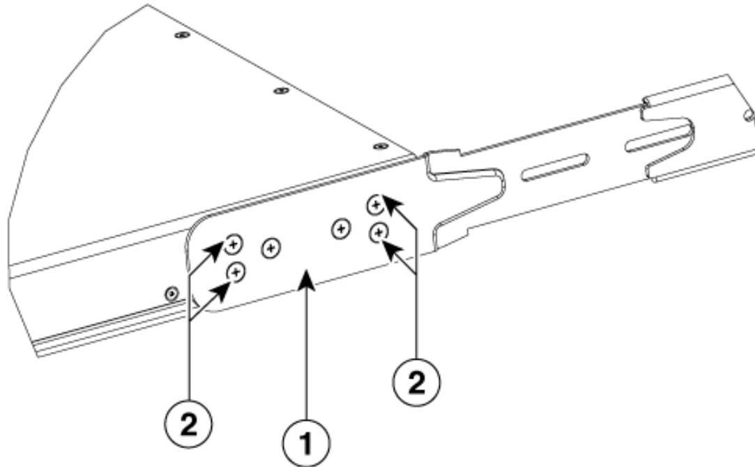
Figure 2: Attaching the Rear Rack-Mount Brackets to the Cisco Catalyst CW9800M Wireless Controller
