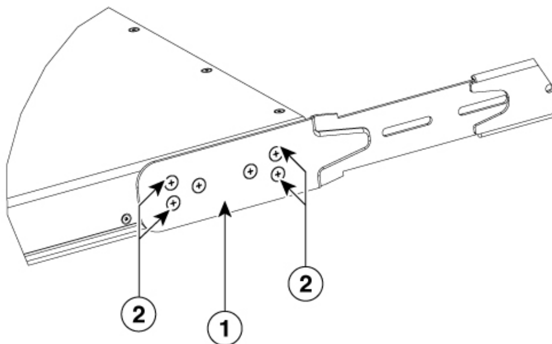
Figure 2: Attaching the Rear Rack-Mount Brackets to the Cisco Catalyst CW9800M Wireless Controller
