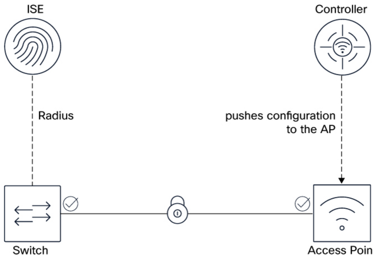
Figure 3: Understanding MACsec IEEE 802.1X
