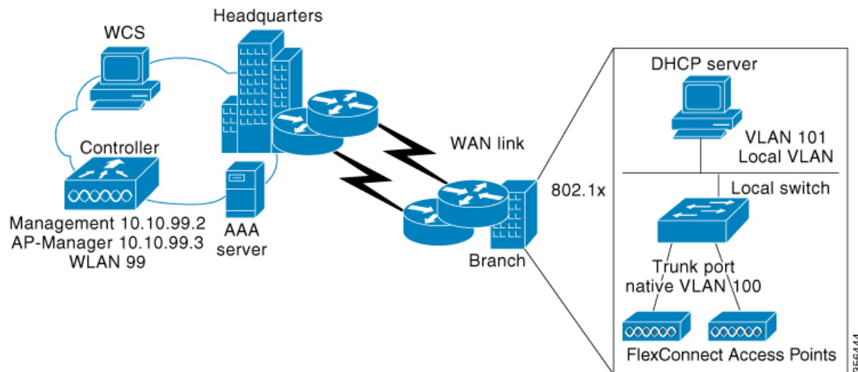
Figure 1: FlexConnect Deployment
