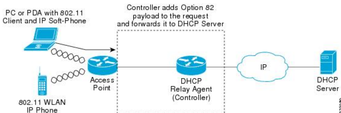
Figure 1: DHCP Option 82
