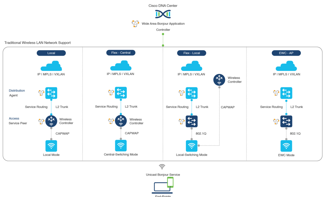
Figure 60: Enterprise Traditional Wireless LAN Network Design
