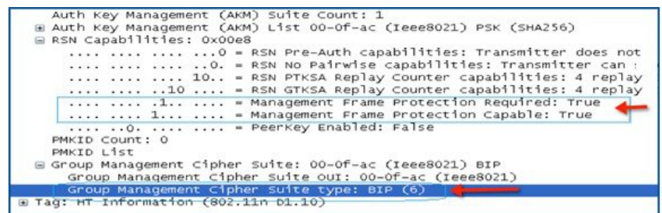
Figure 34: 802.11w Information Elements
