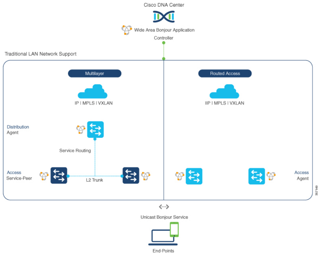
Figure 59: Enterprise Wired Multilayer and Routed Access Network Design
