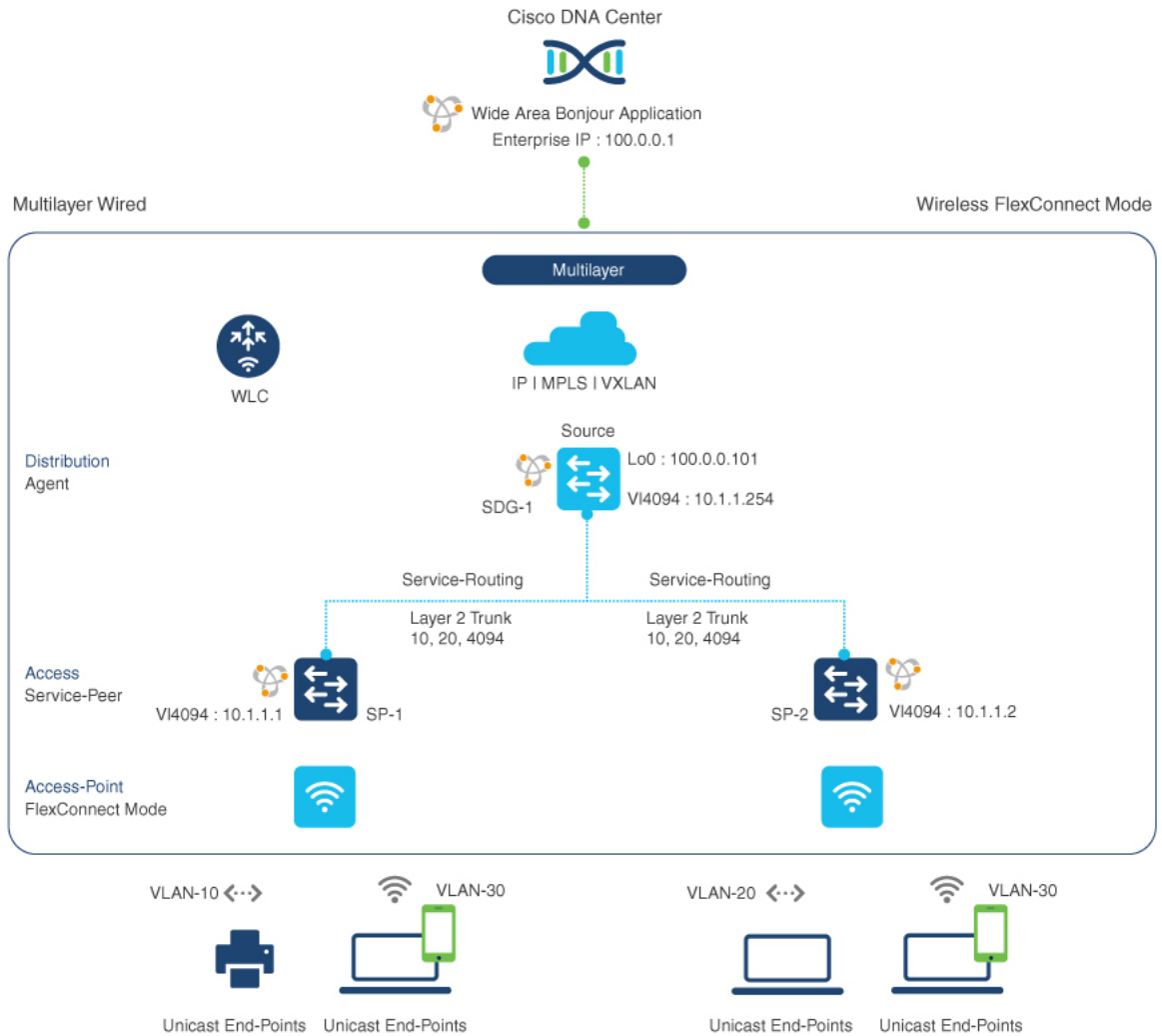
Figure 1: Local Area Bonjour Service-Routing Multilayer Wired and Wireless FlexConnect Local-Switching Mode
