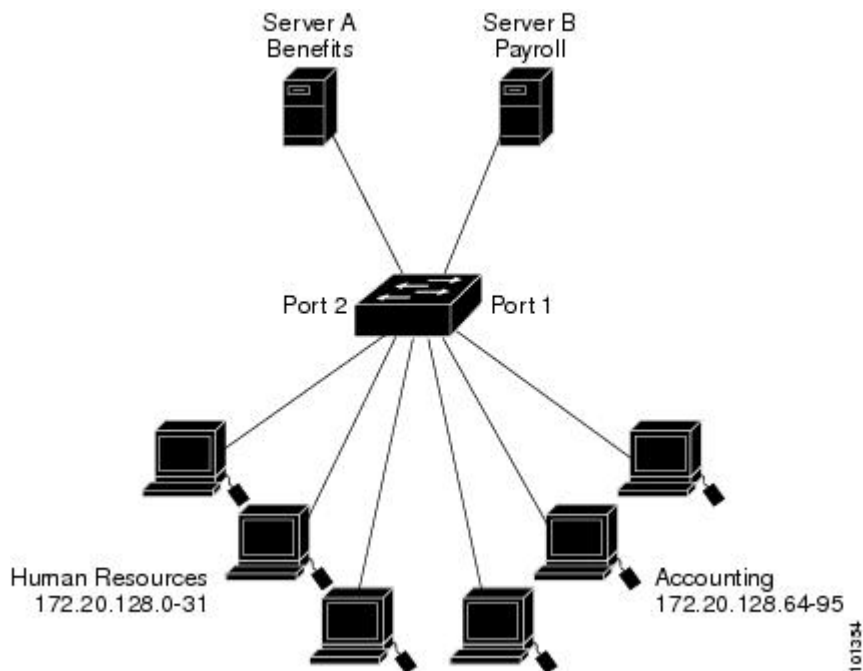
Figure 38: Using Router ACLs to Control Traffic
