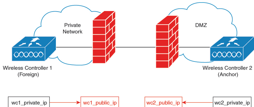
Figure 45: Mobility NAT
