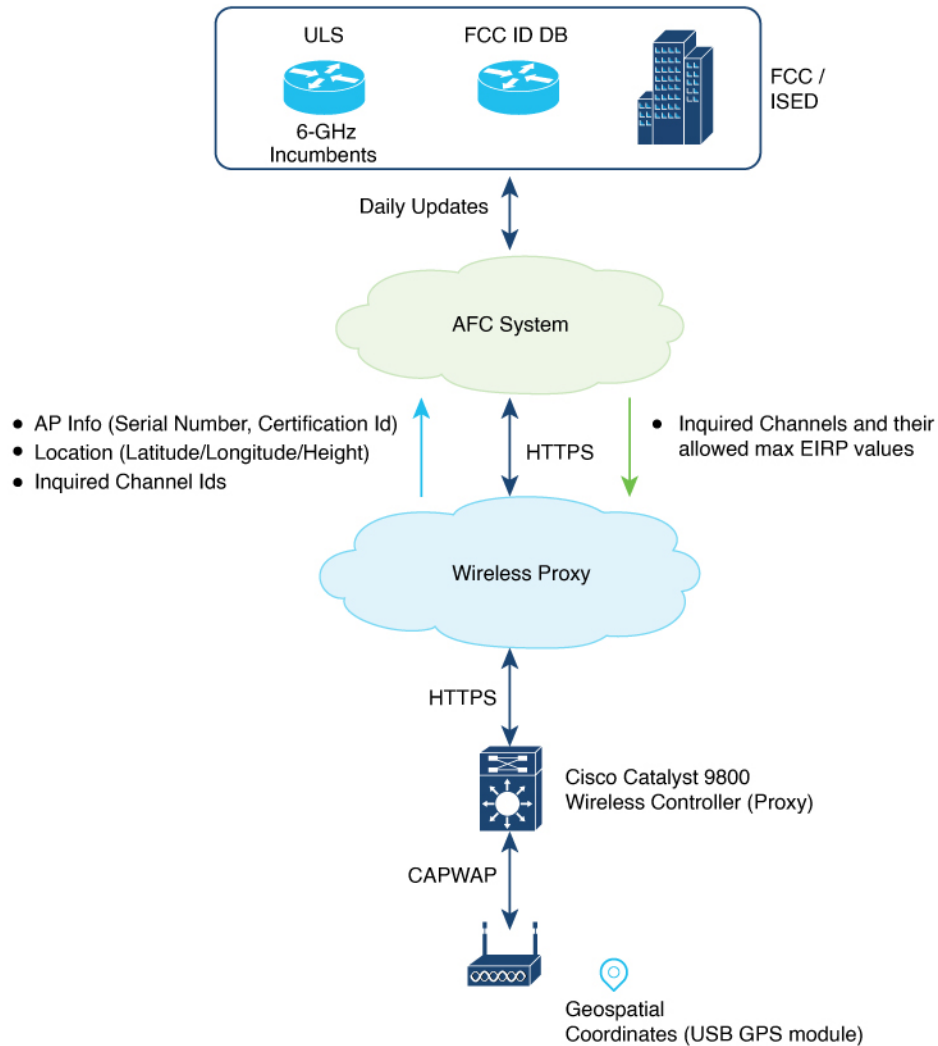
Figure 59: AFC Architecture
