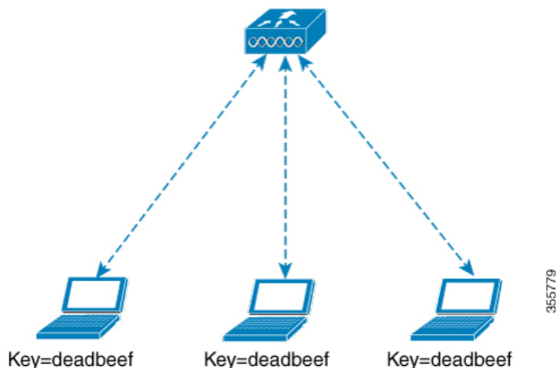
Figure 30: Traditional PSK
