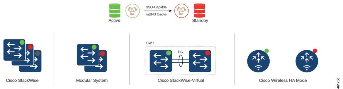
Figure 70: mDNS Service-Gateway SSO
