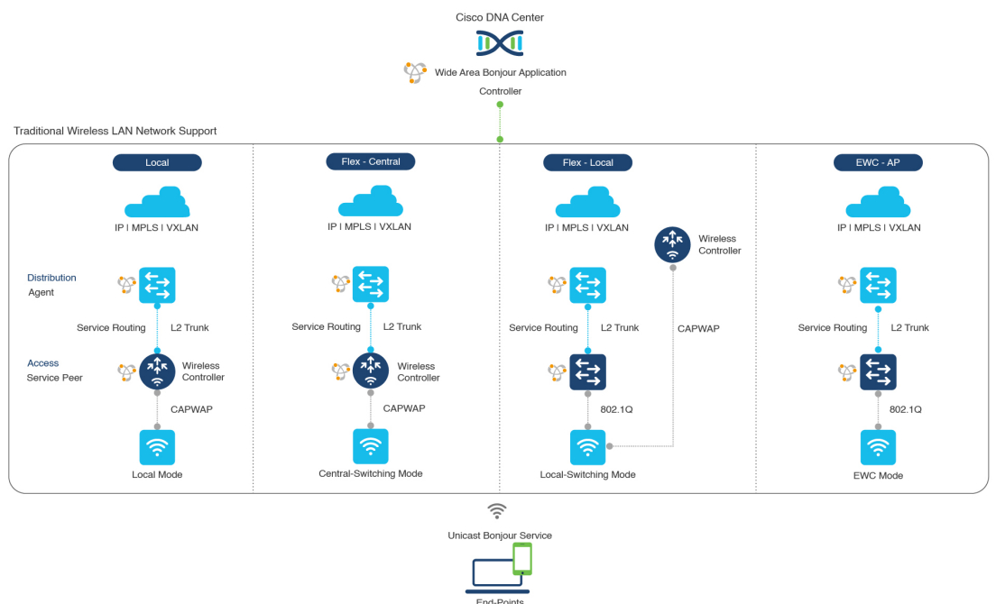
Figure 62: Enterprise Traditional Wireless LAN Network Design
