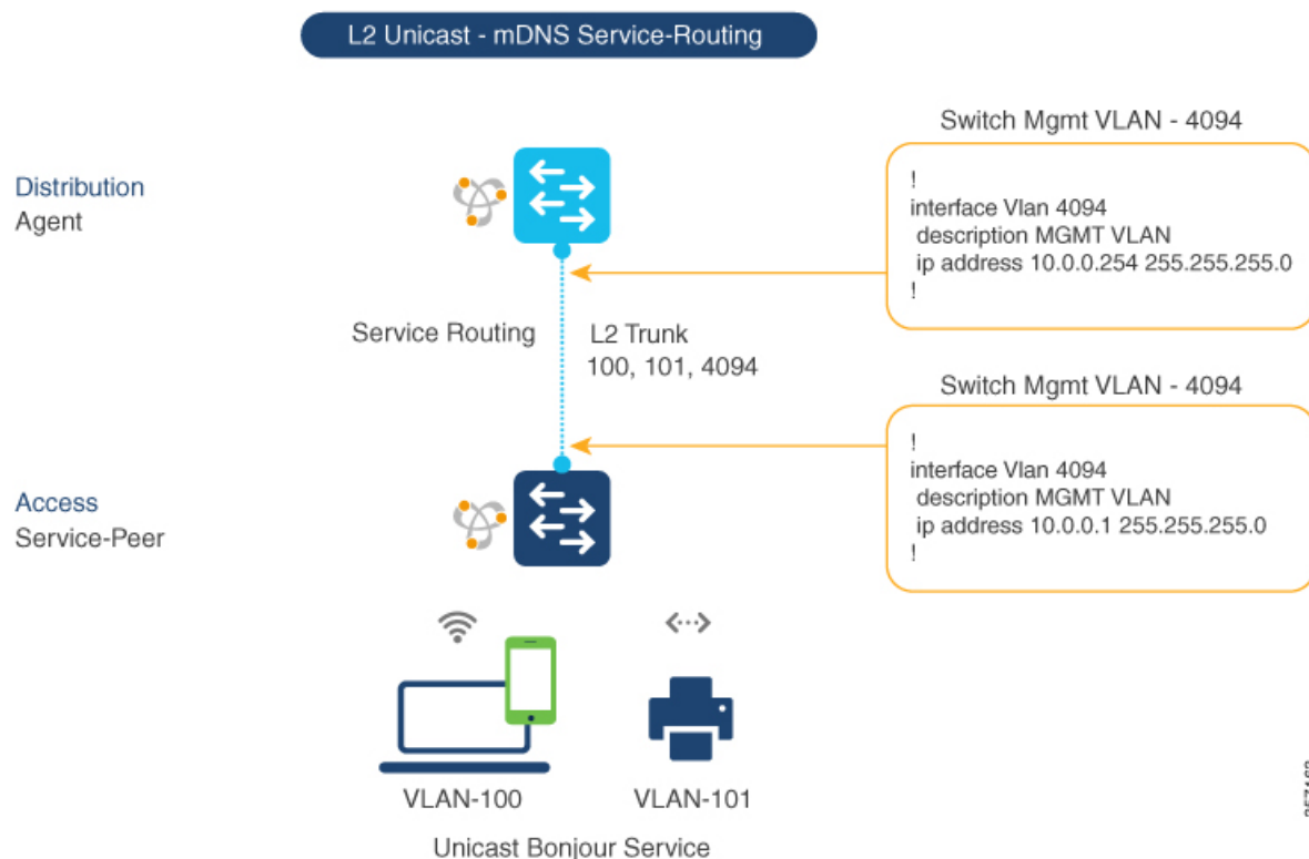
Figure 78: Catalyst Service-Peer Service-Routing Configuration
