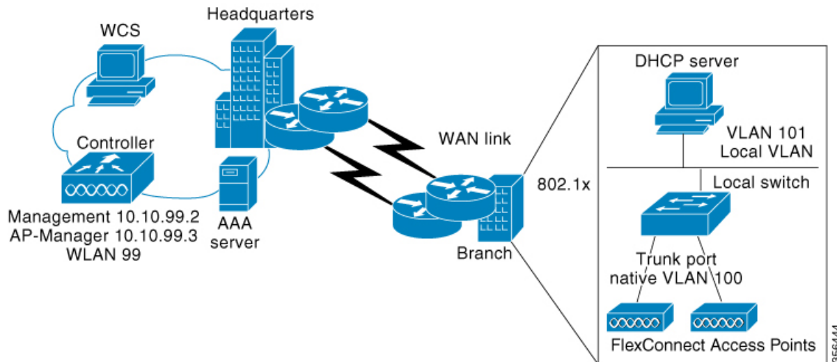
Figure 16: FlexConnect Deployment
