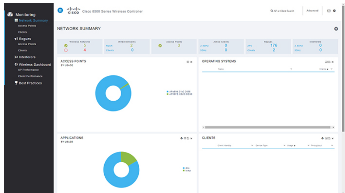
Figure 1: Monitoring Dashboard
