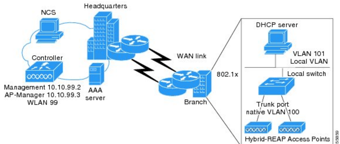
Figure 1: FlexConnect Deployment
