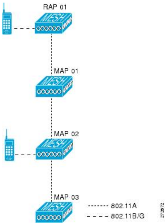
Figure 20: Mesh Network Example
