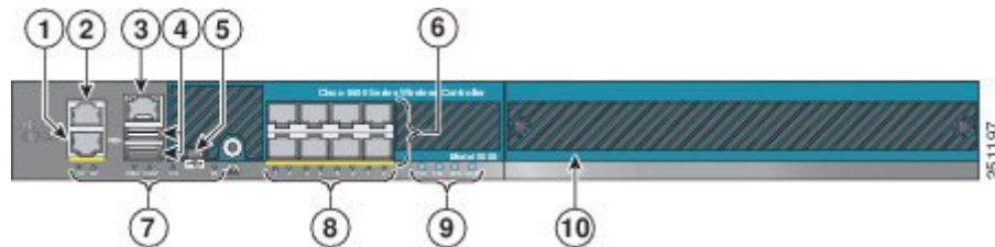
Figure 1: Ports on the Cisco 5508 Wireless Controllers
