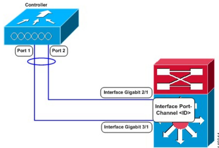
Figure 2: Link Aggregation LAG with the Catalyst 6500 Series Neighbor Switch
