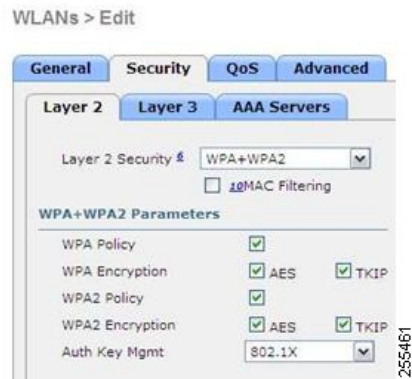
Figure 7: Compatible Security Settings for OEAP Series
