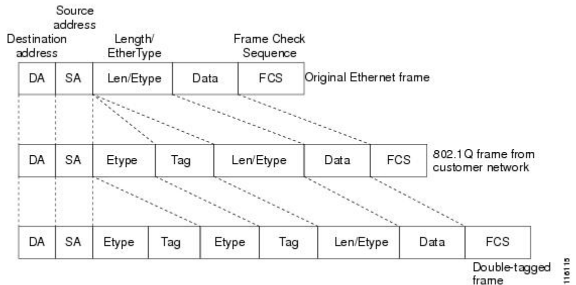
Figure 1: Untagged 802.1Q-Tagged and 802.1Q-in-Q Tagged Ethernet Frames
