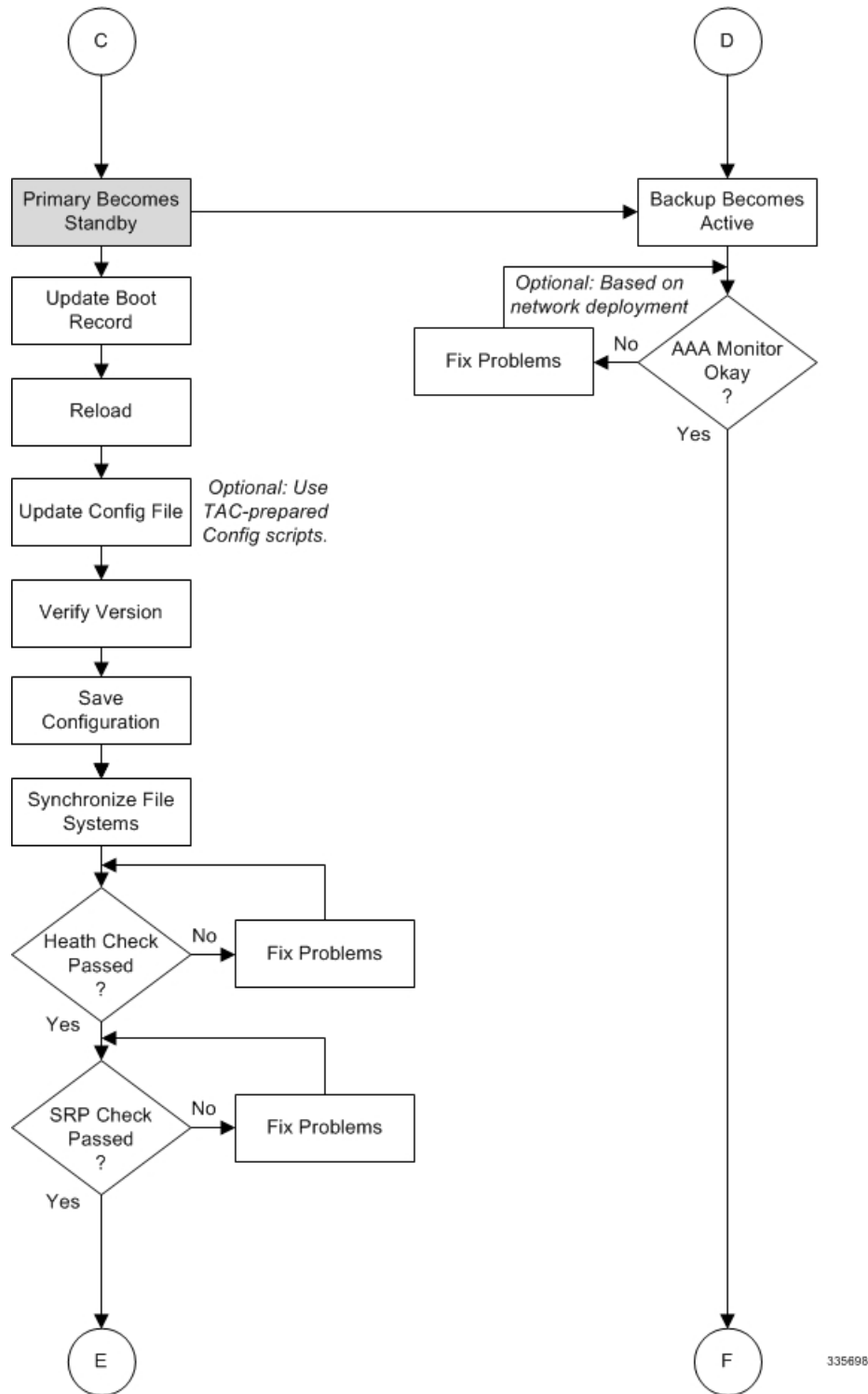
Figure 8: ICSR Software Upgrade – Part 4
