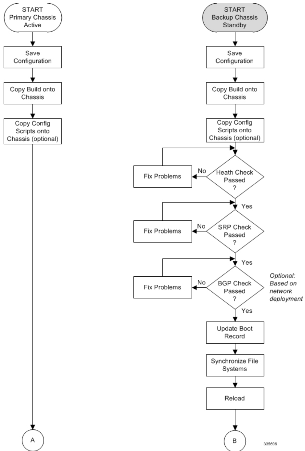
Figure 6: ICSR Software Upgrade – Part 2
