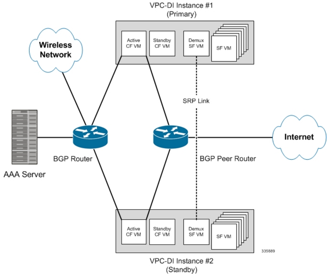
Figure 1: VPC-DI ICSR Network
