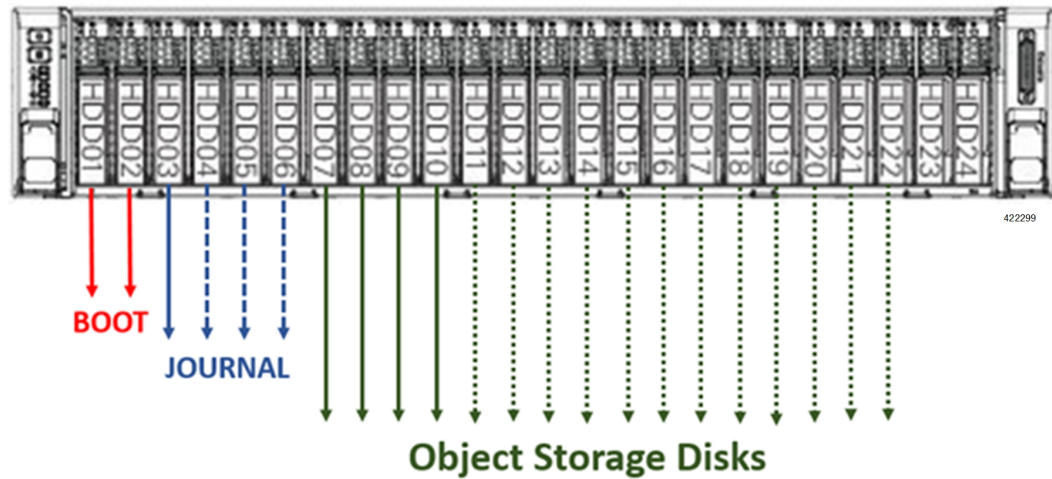
Figure 1: UCS C240 Front-Plane
