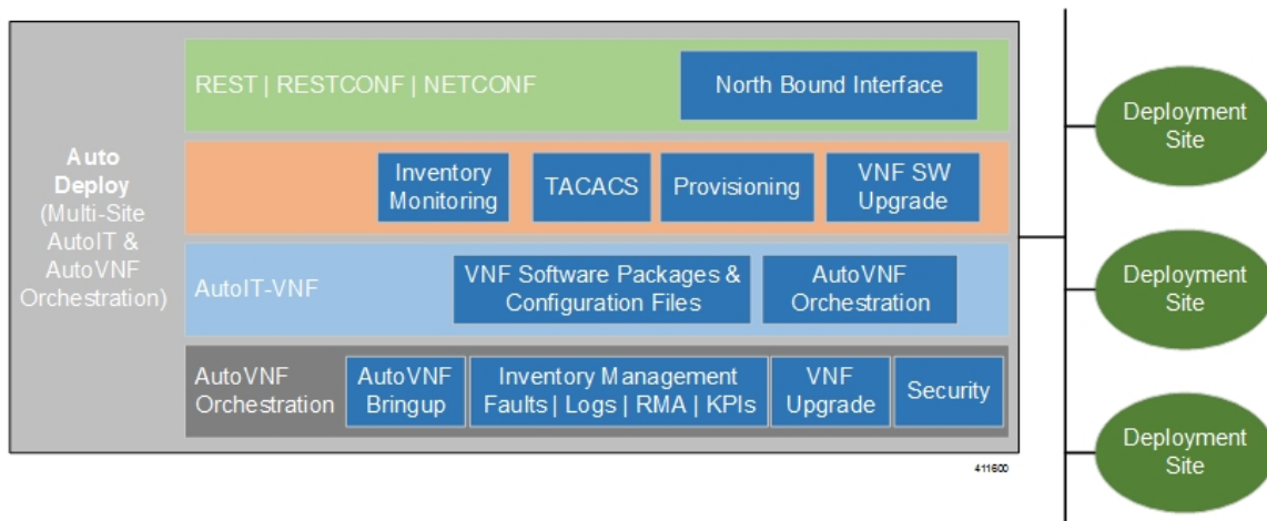
Figure 5: AutoDeploy Functions
