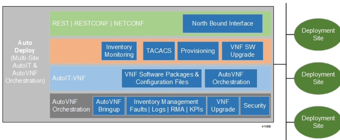
Figure 5: AutoDeploy Functions
