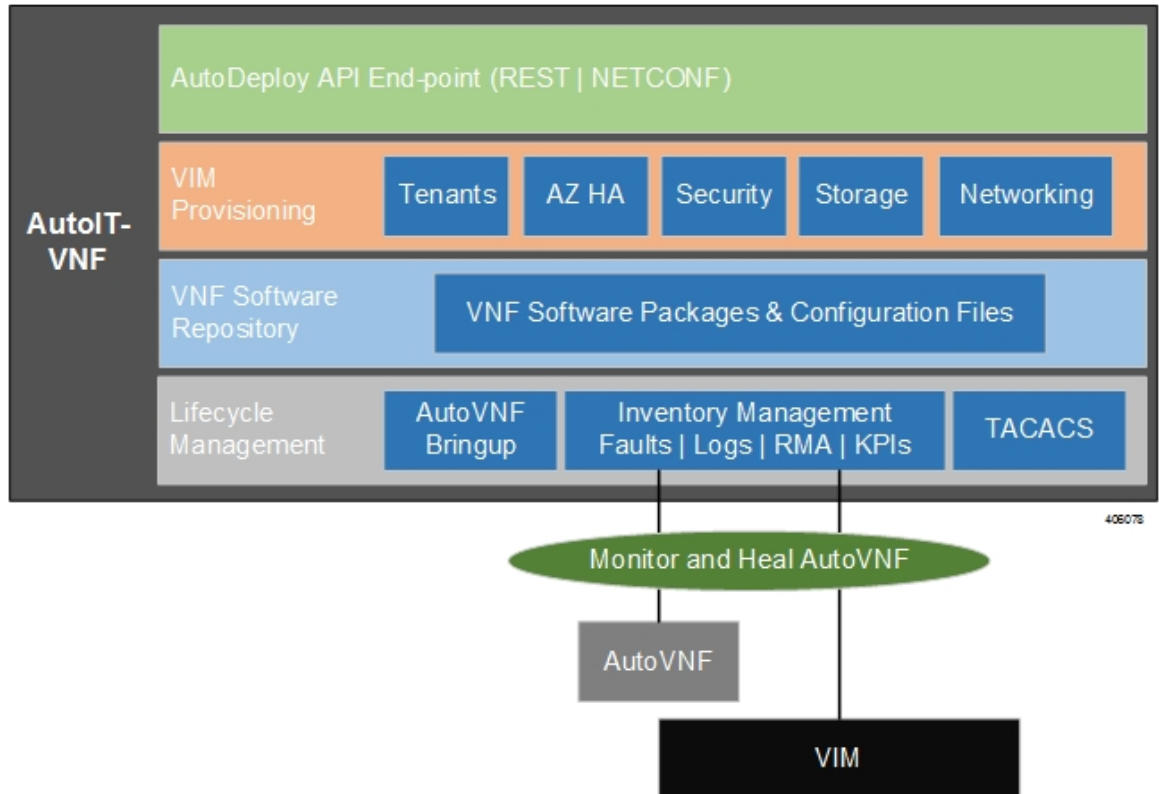
Figure 4: AutoIT-VNF Functions
