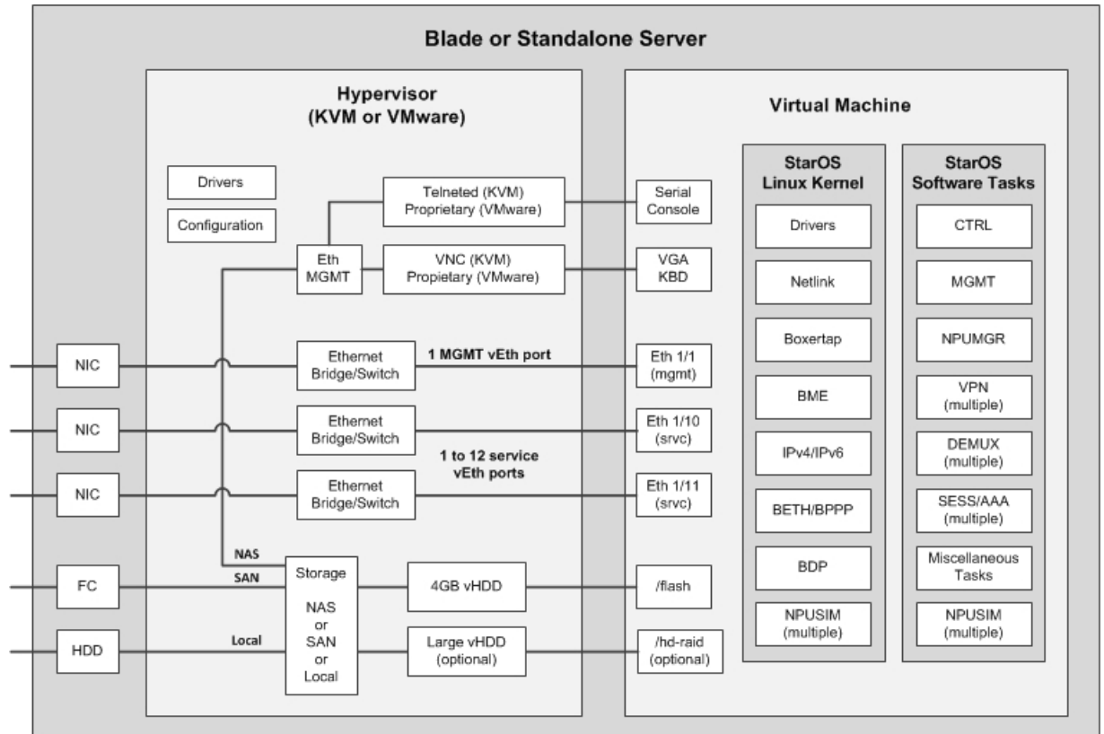
Figure 2: VPC-SI Overview
