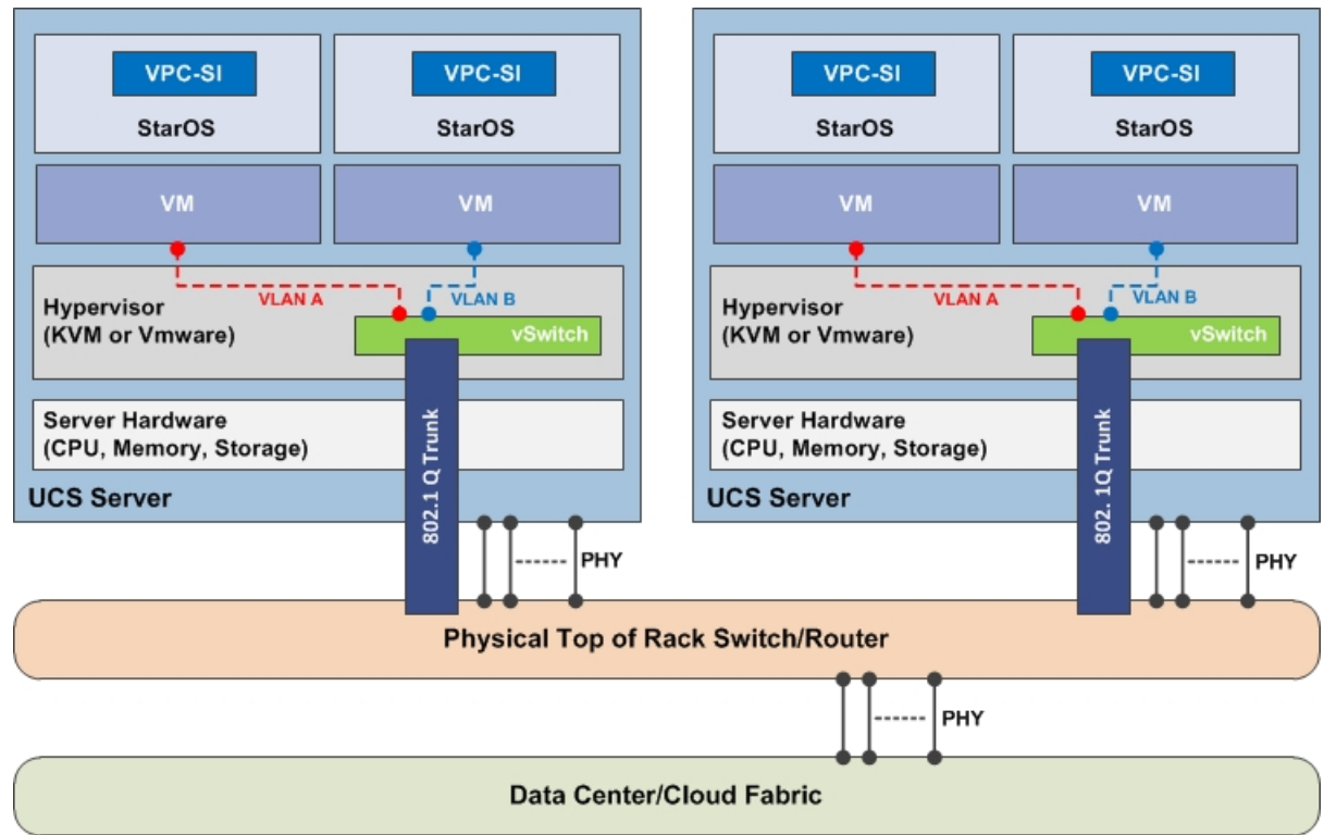
Figure 1: L2/L3 Interconnection
