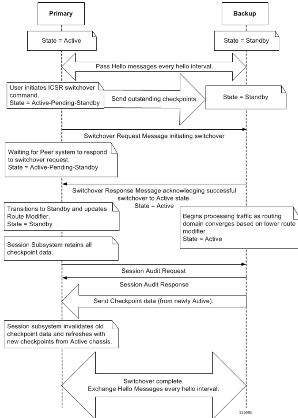
Figure 10: ICSR Process Flow (Manual Switchover)
