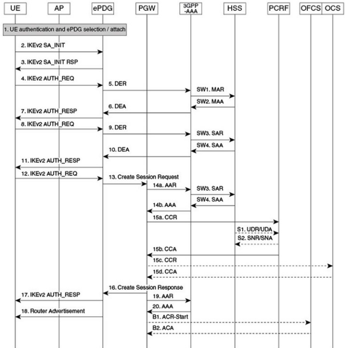
Figure 33: Call Flow of P-GW/SMF Gateway Selection
