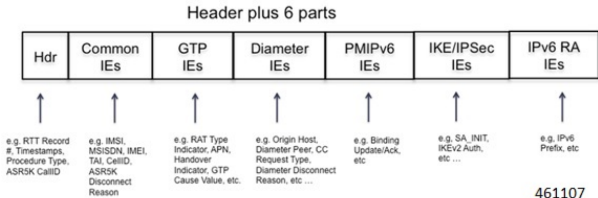
Figure 23: RTT Record Schema
