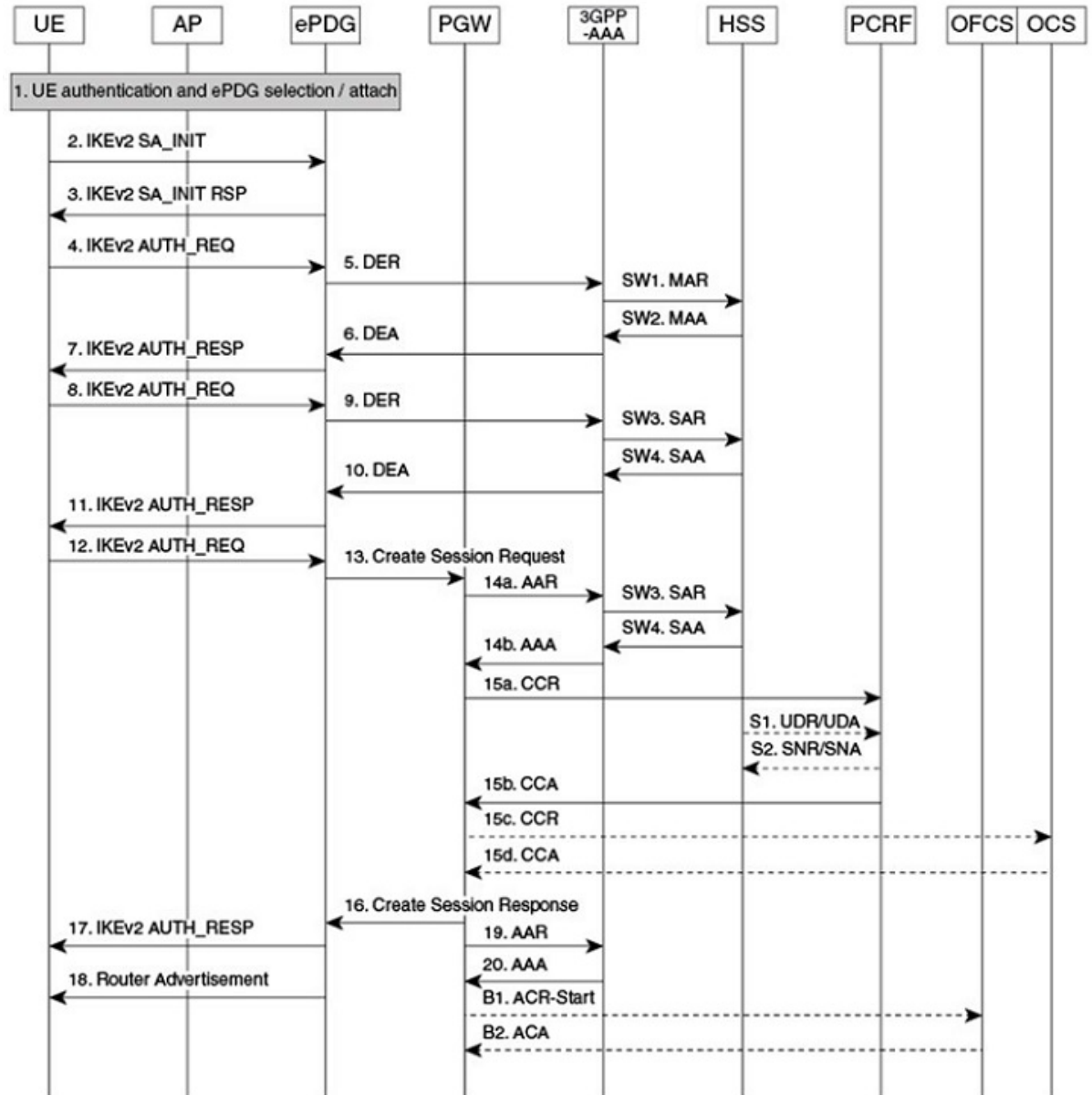
Figure 29: ePDG Setup Procedure Call Flow
