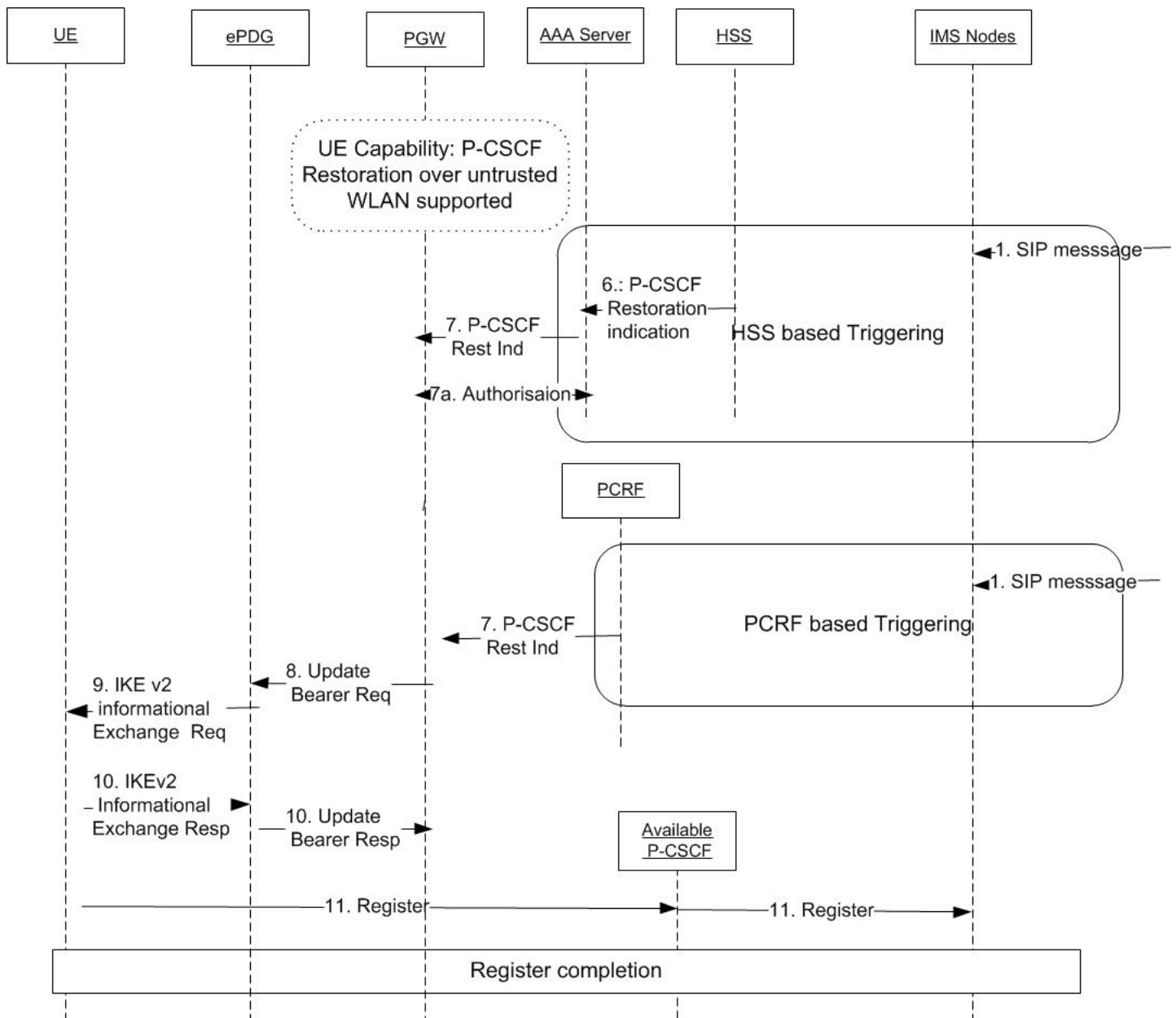
Figure 28: PCRF Based Extended P-CSCF Restoration for Un-Trusted WLAN Access
