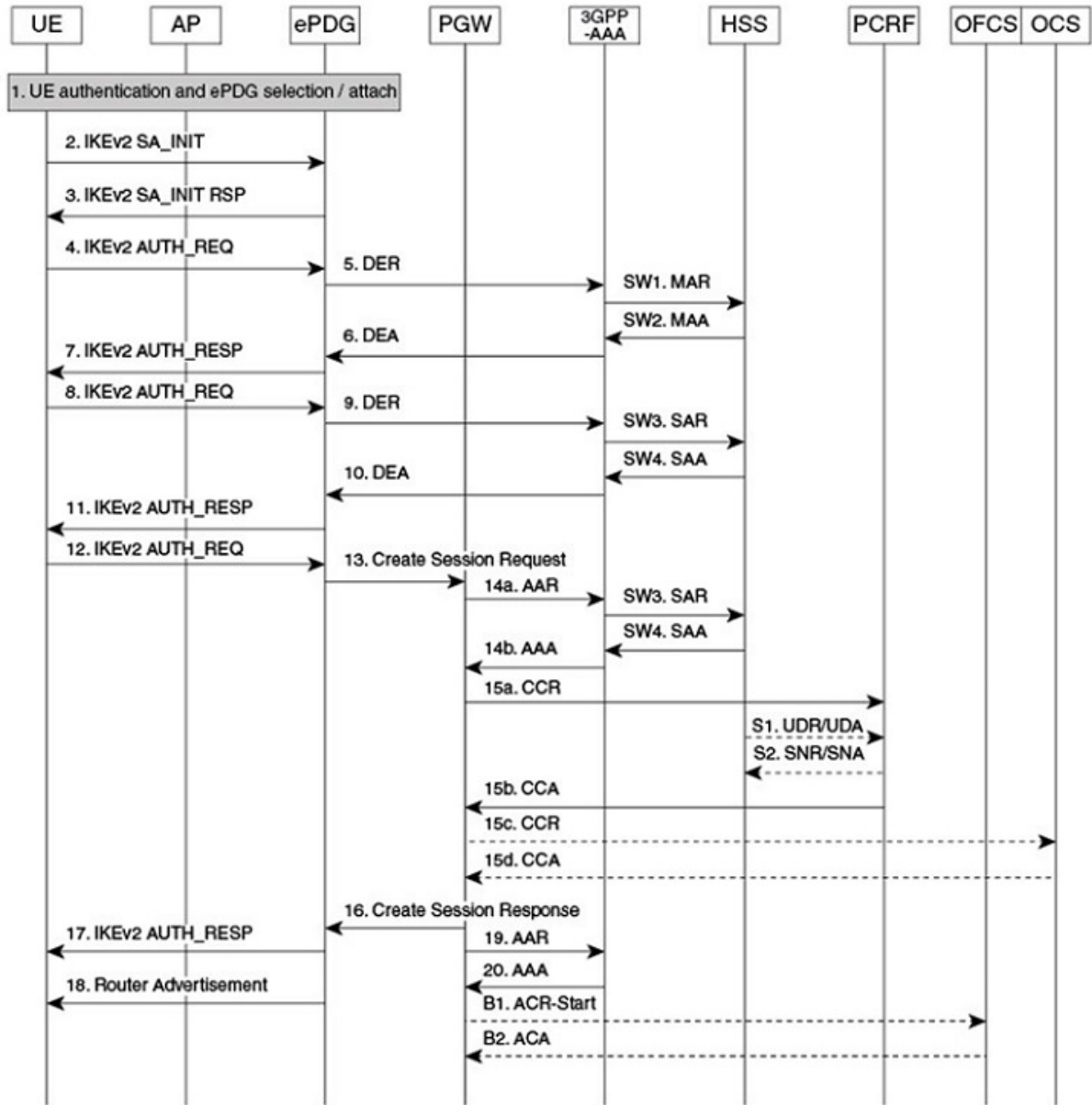
Figure 24: ePDG Setup Procedure Call Flow
