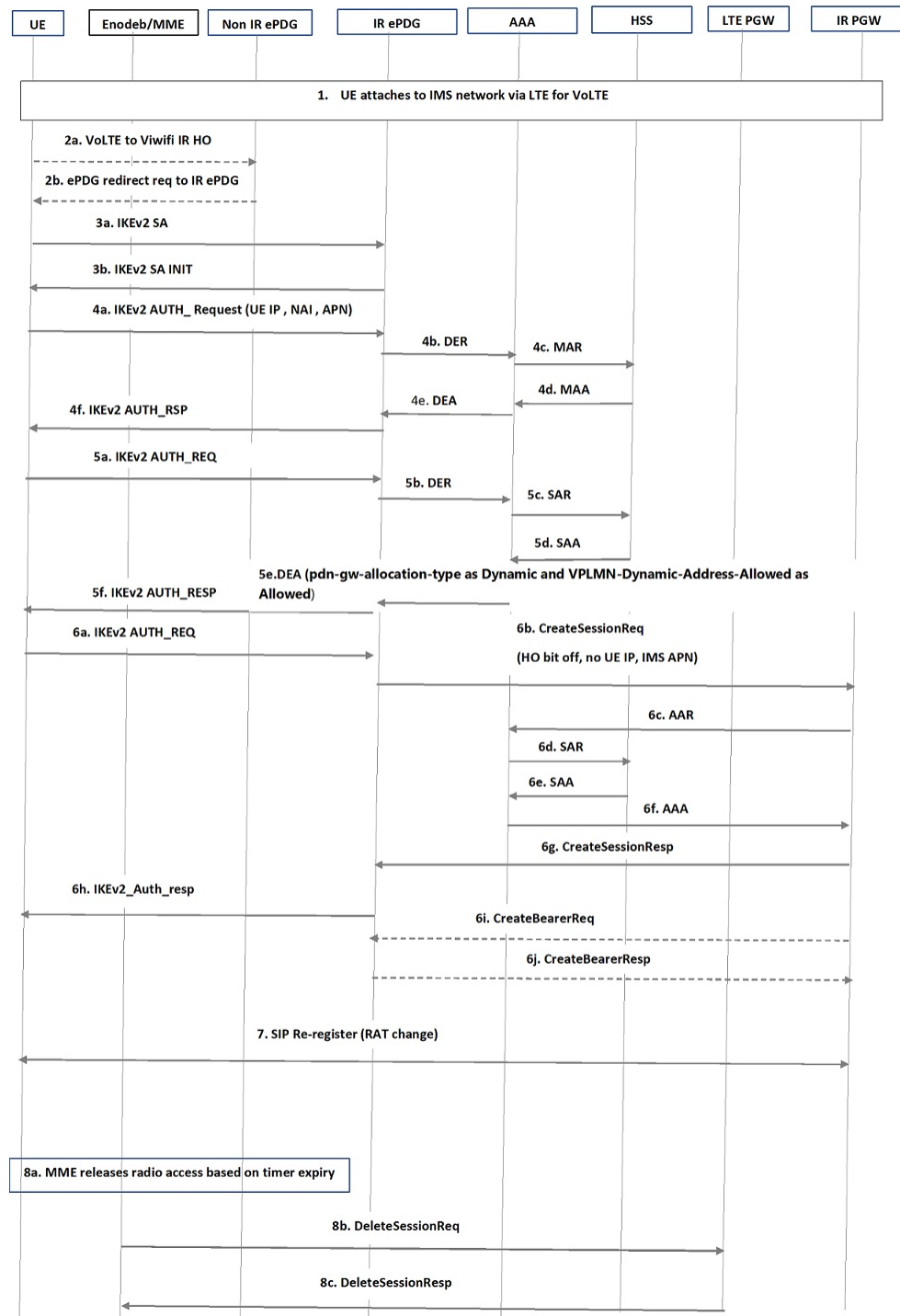
Figure 26: VoLTE to VoWi-Fi IR HO to IR ePDG
