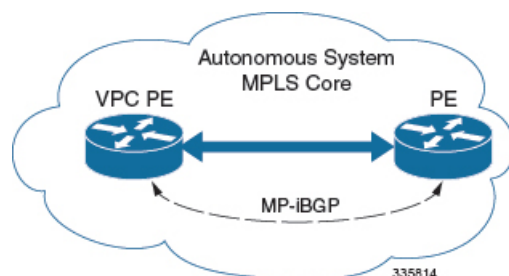
Figure 2: VPC-DI as a PE
