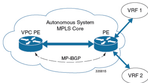
Figure 3: Sample Configuration
