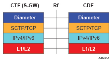
Figure 11: Supported Protocols on the Rf Interface
