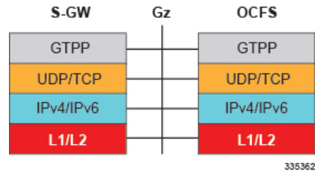
Figure 10: Supported Protocols on the Gz Interface
