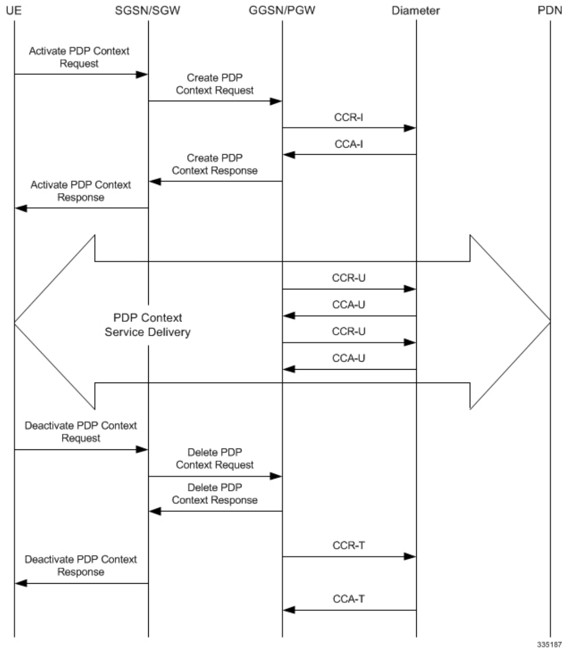
Figure 3: Gy Call Flow for Simple Call Request for GGSN/P-GW/IPSG
