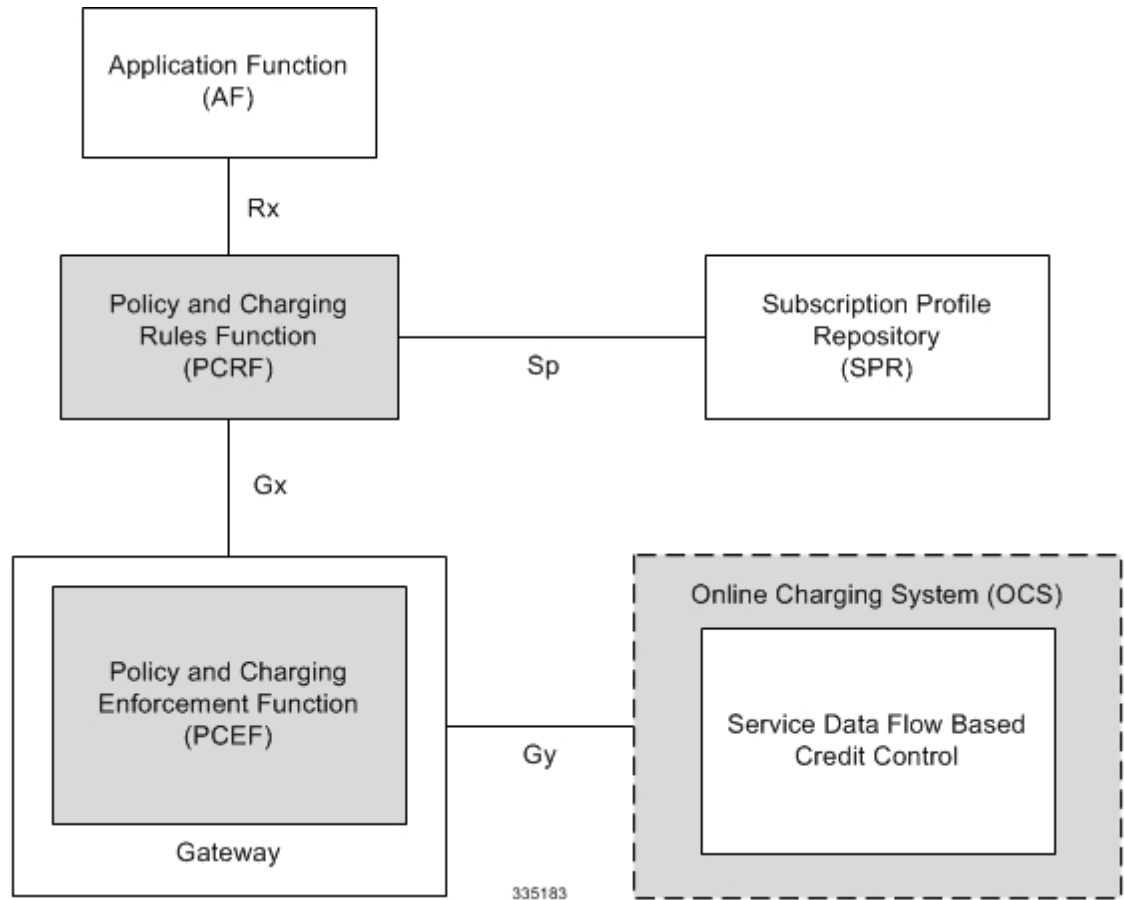
Figure 11: HA/PDSN Rel. 8 Gx PCC Logical Architecture
