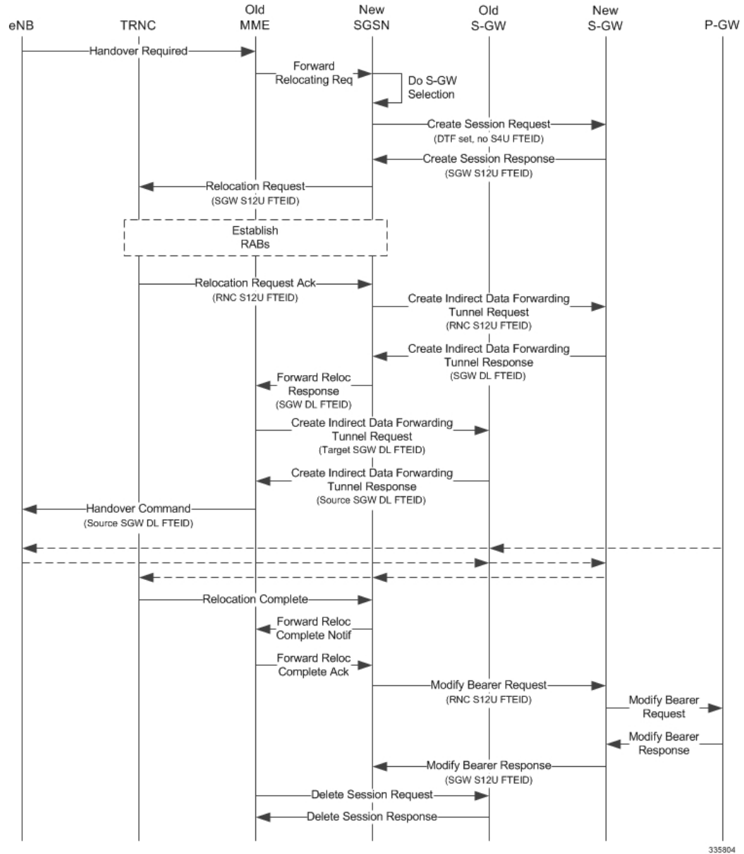
Figure 31: New SRNS with S-GW Change and Indirect Data Transfer
