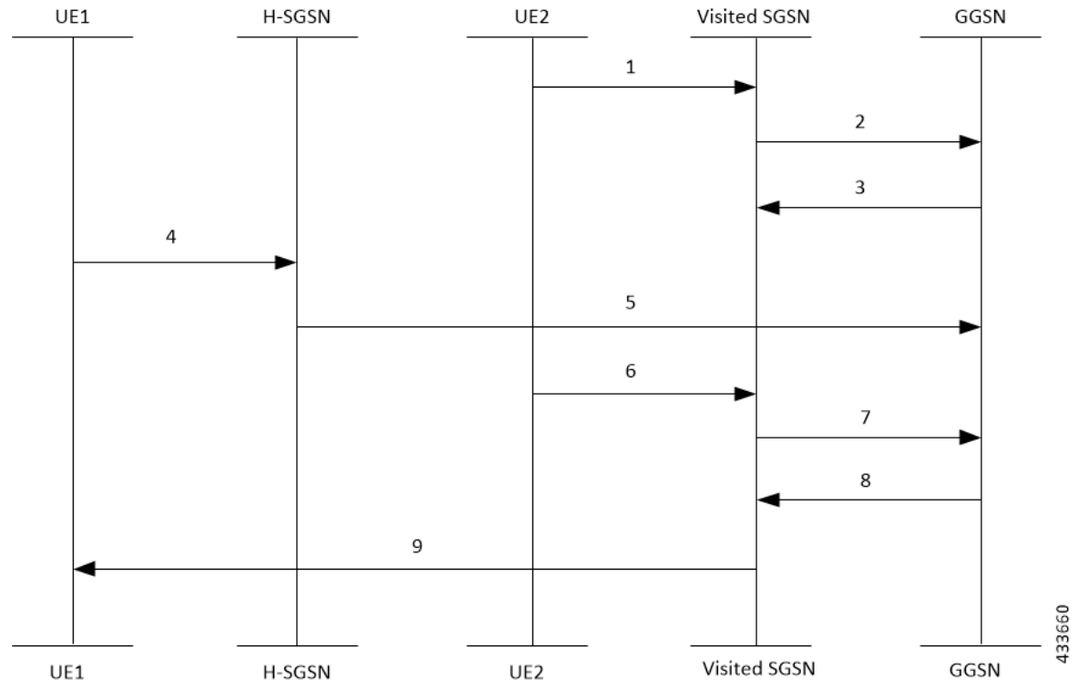
Figure 116: GTPC-Based TEID Collision Detection as per ULI Change
