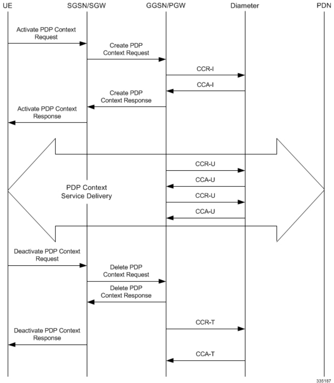
Figure 67: Gy Call Flow for Simple Call Request for GGSN/P-GW/IPSG
