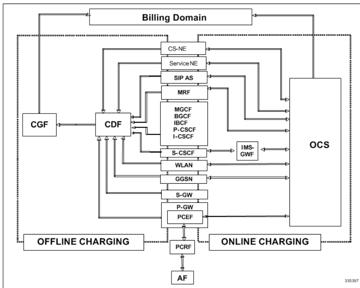
Figure 108: Charging Architecture
