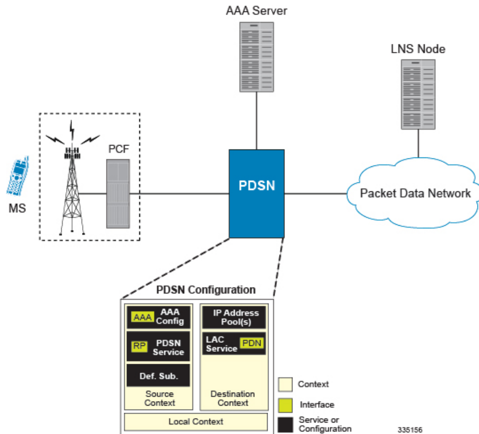
Figure 85: LAC Service Configuration for SIP
