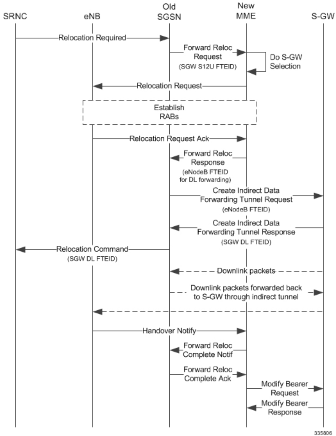
Figure 33: Old SRNS with Indirect Data Transfer 4
