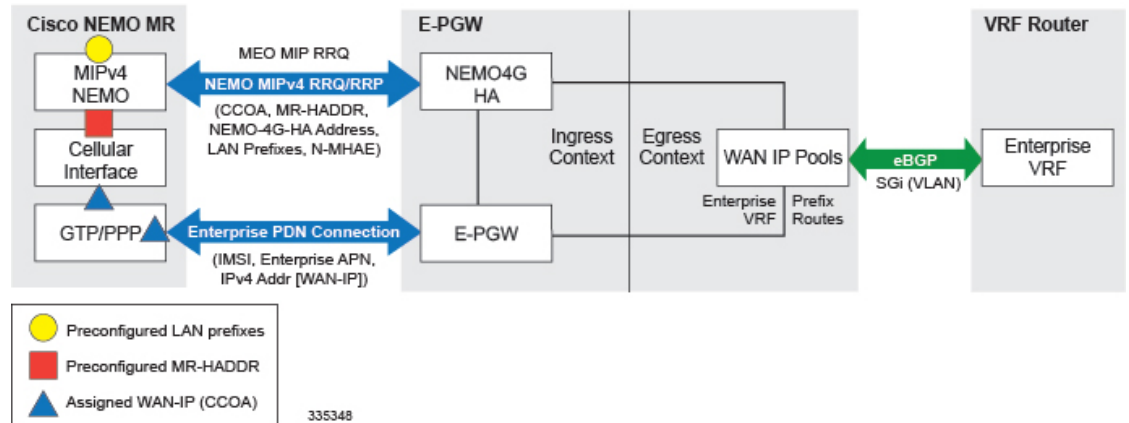
Figure 97: NEMO Control Plane
