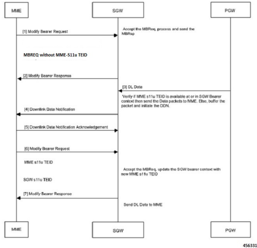
Figure 77: Call Flow for Handling IE Validation at EGTP Protocol
