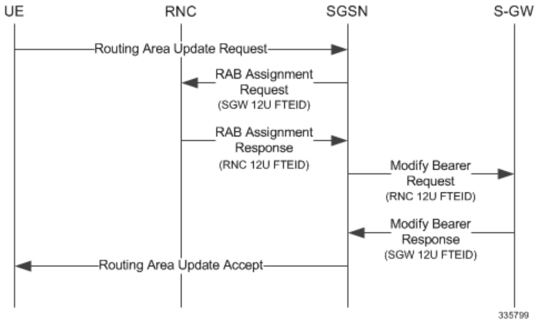
Figure 26: Routing Area Update Procedure without SGW Change
