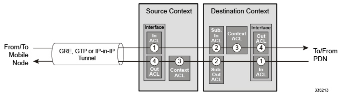
Figure 1: ACL Processing Order
