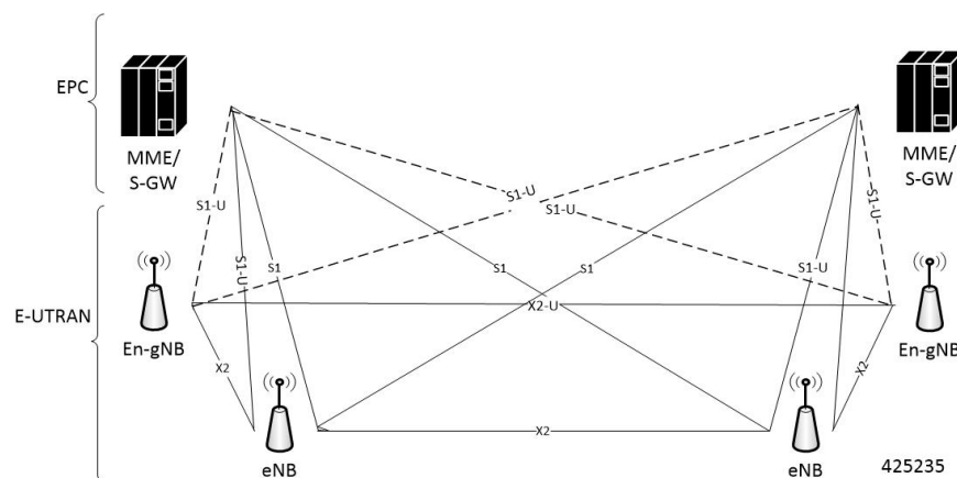
Figure 1: EN-DC Architecture
