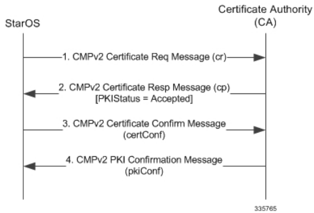
Figure 7: Call Flow: Successful Enrollment Request
