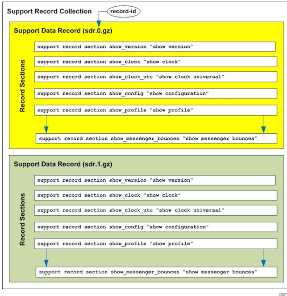
Figure 2: Support Data Collection Hierarchy
