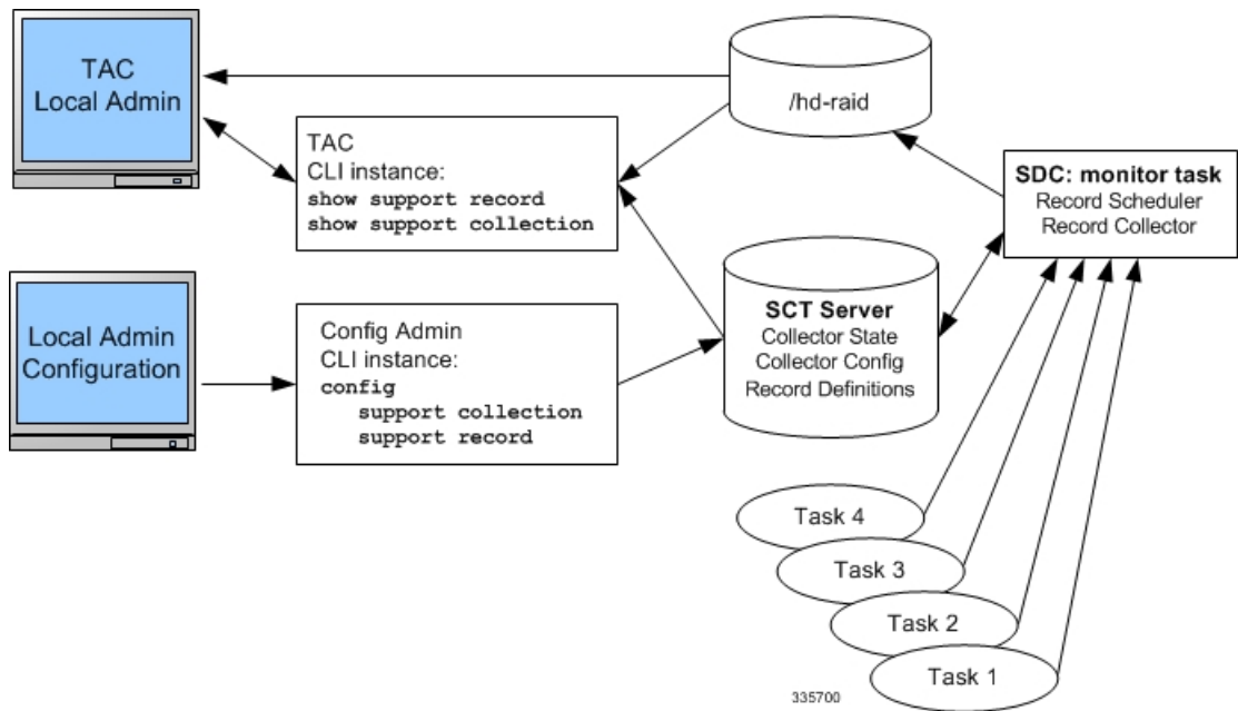
Figure 1: SDC Tasks and Processes&lt;
