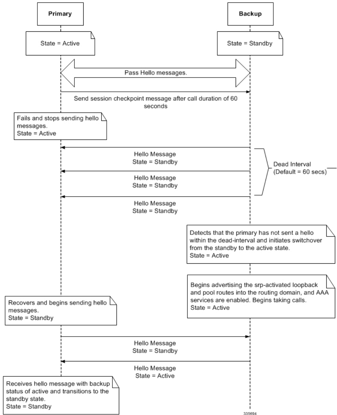
Figure 1: ICSR Process Flow (Primary Failure)
