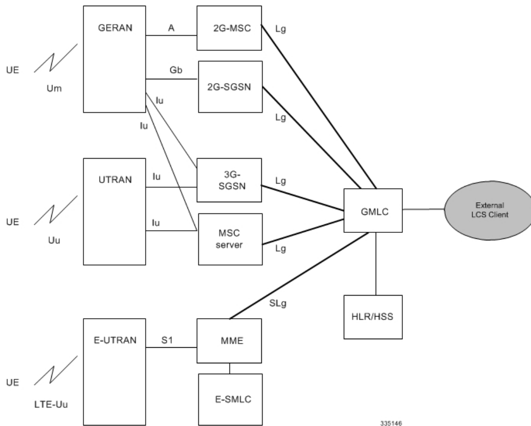
Figure 1: LCS Architecture
