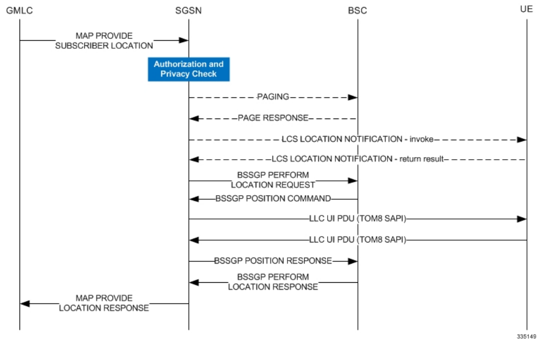
Figure 2: 2G Mobile Terminating Location Request
