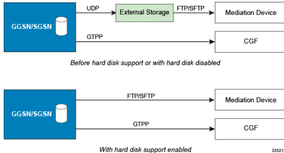
Figure 1: HDD Mechanism
