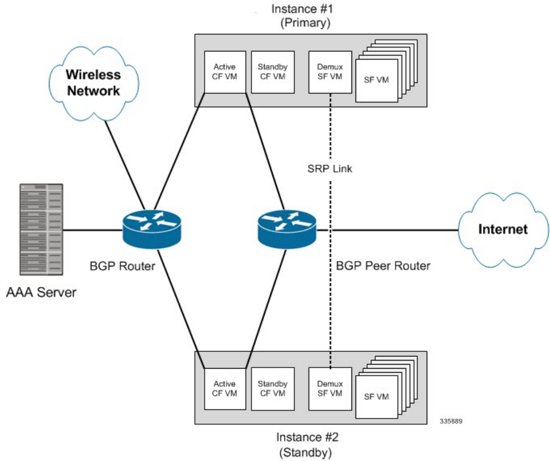
Figure 2: Virtualized StarOS ICSR Network
