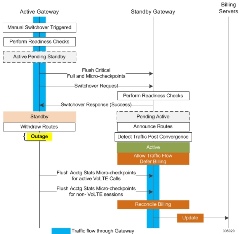
Figure 5: Call Flow: Reduce Non-VoLTE Data Outage
