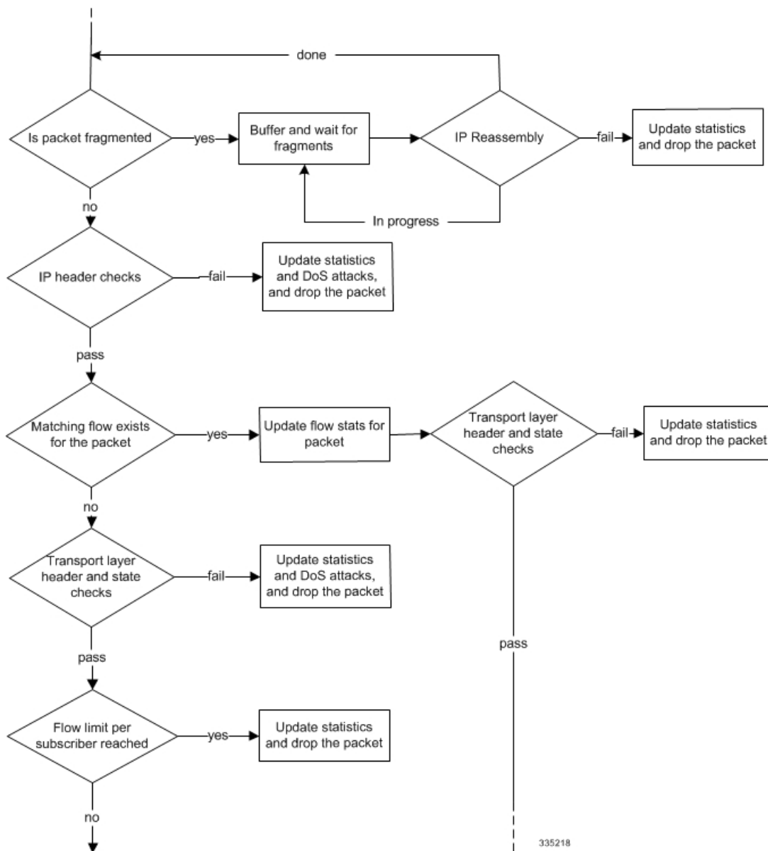
Figure 4: ...NAT Processing Flow
