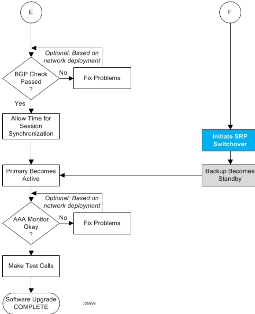
Figure 7: ICSR Software Upgrade – Part 4
