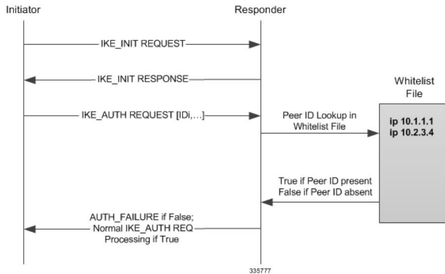
Figure 2: Whitelist Implementation
