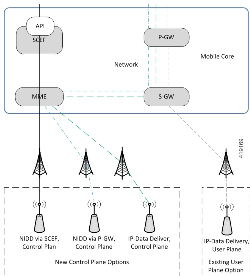
Figure 1: Control Plane Architecture for Small Data Delivery
