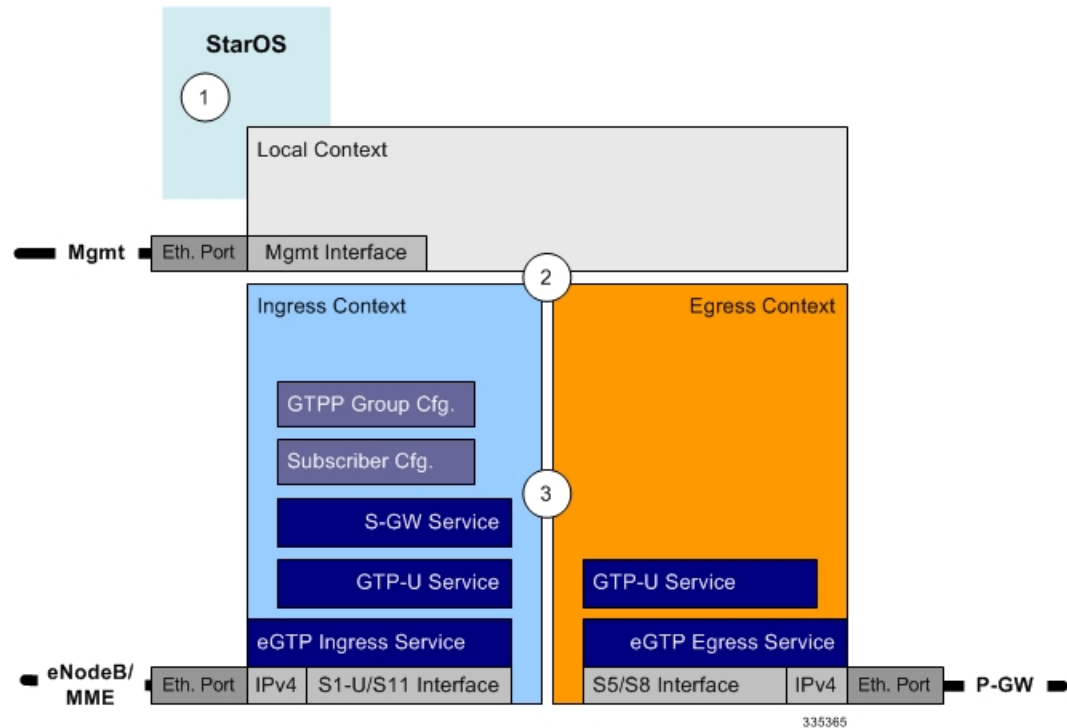
Figure 2: eGTP S-GW Configurable Components
