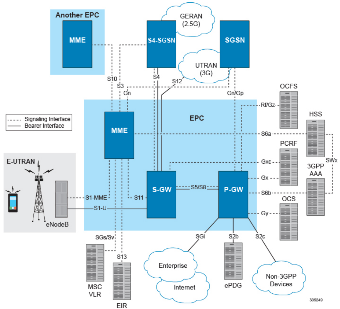
Figure 16: P-GW in the E-UTRAN/EPC Network
