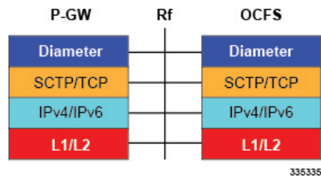
Figure 25: Protocols Supported on the Rf Interface
