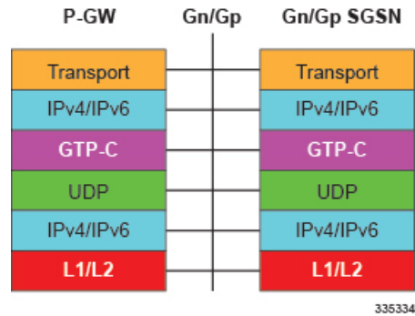
Figure 24: Protocols Supported on the Gn/Gp Interface
