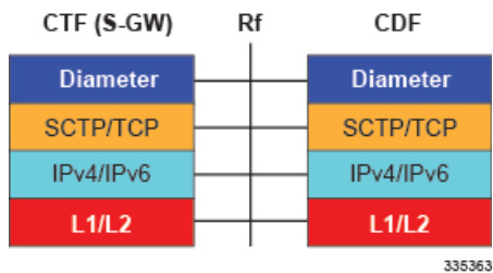
Figure 14: Protocols Supported on the Rf Interface
