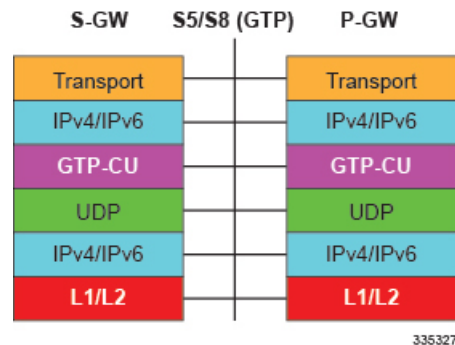
Figure 28: Protocols Supported on the GTP P-GW S5/S8 Interface
