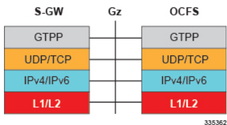
Figure 13: Protocols Supported on the Gz Interface
