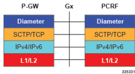
Figure 21: Protocols Supported on the Gx Interface
