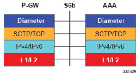
Figure 30: Protocols Supported on the S6b Interface
