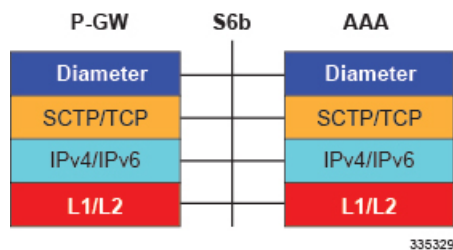
Figure 19: Supported Protocols on the S6b Interface
