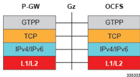
Figure 23: Protocols Supported on the Gz Interface
