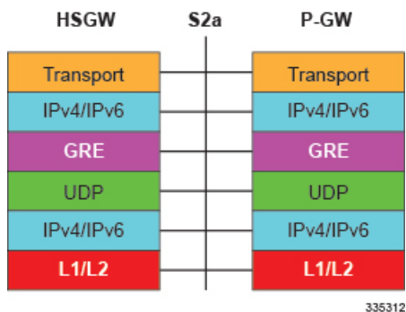
Figure 29: Protocols Supported on the S2a Interface
