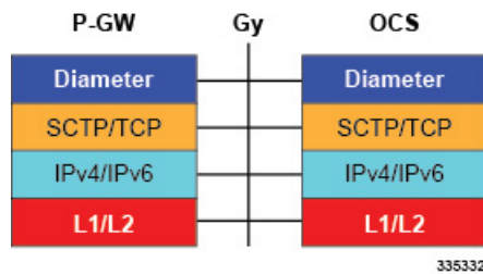
Figure 22: Protocols Supported on the Gy Interface
