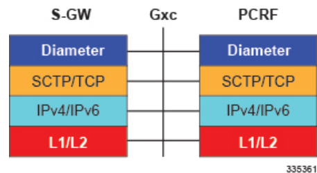
Figure 12: Supported Protocols on the Gxc Interface
