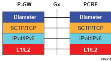
Figure 32: Protocols Supported on the Gx Interface
