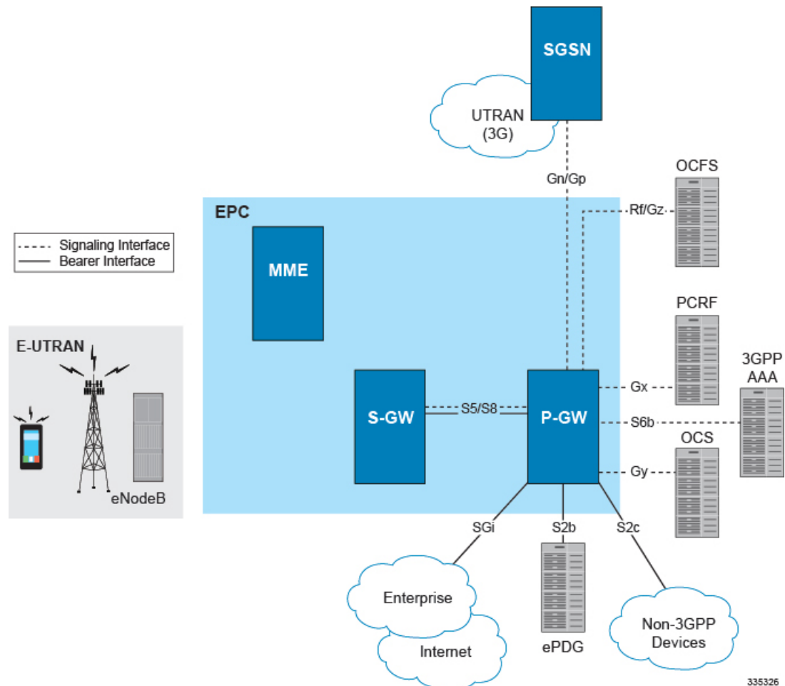
Figure 15: Supported P-GW Interfaces in the E-UTRAN/EPC Network
