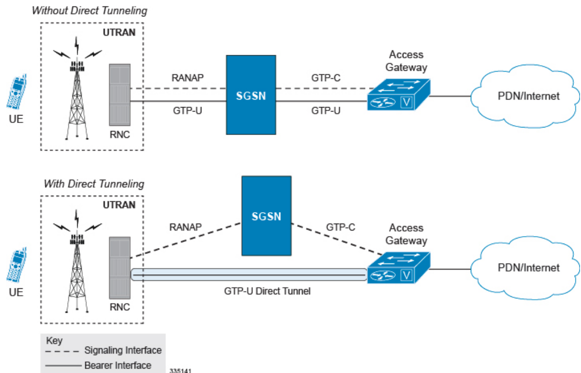
Figure 35: GTP-U with Direct Tunnel
