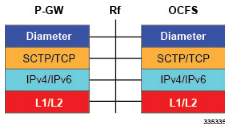
Figure 33: Protocols Supported on the Rf Interface
