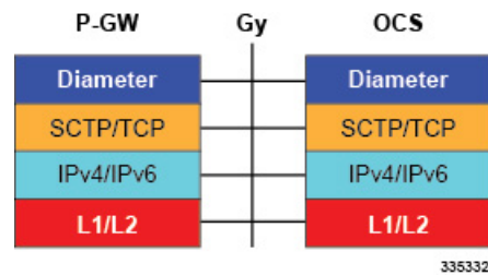
Figure 34: Protocols Supported on the Gy Interface
