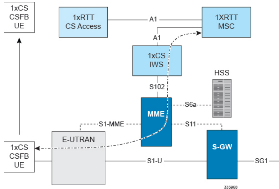
Figure 1: Architecture of the MME s CSFB for 1xRTT
