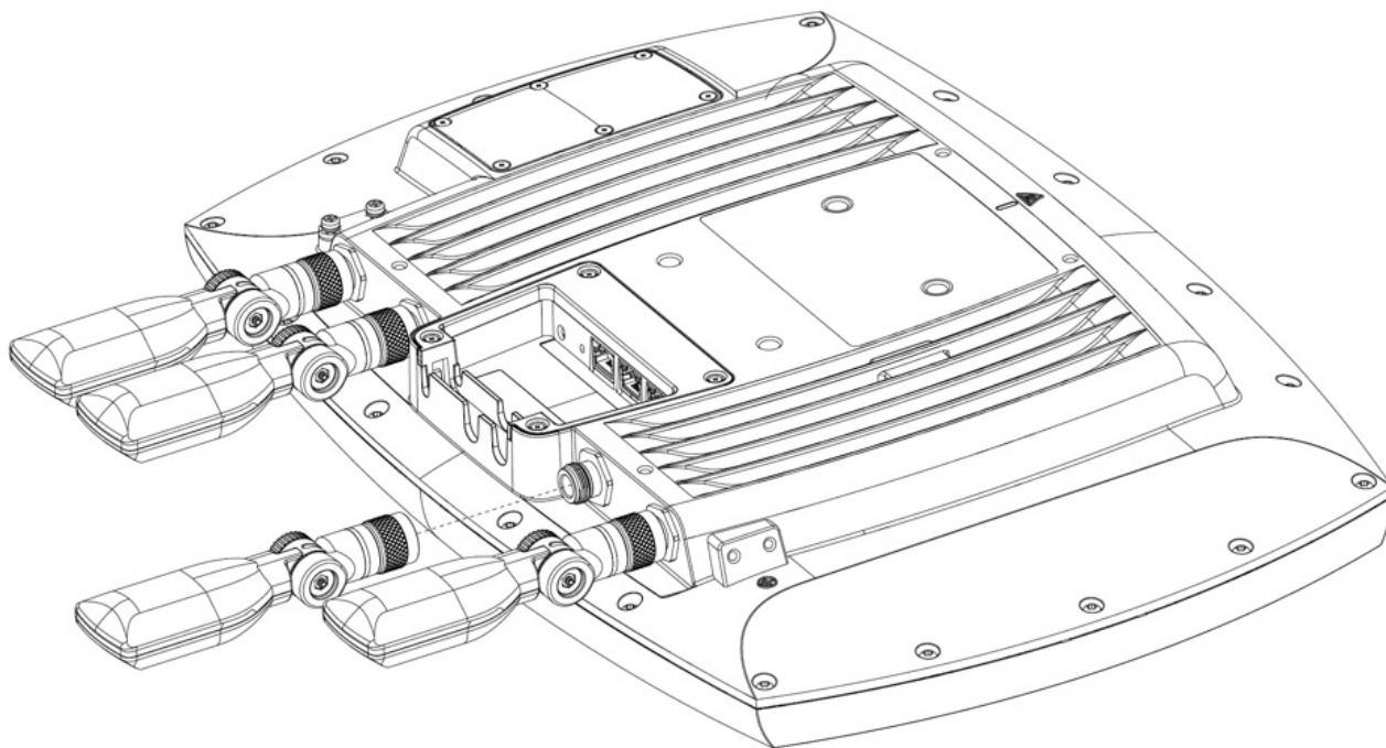
Figure 7: Align antenna
